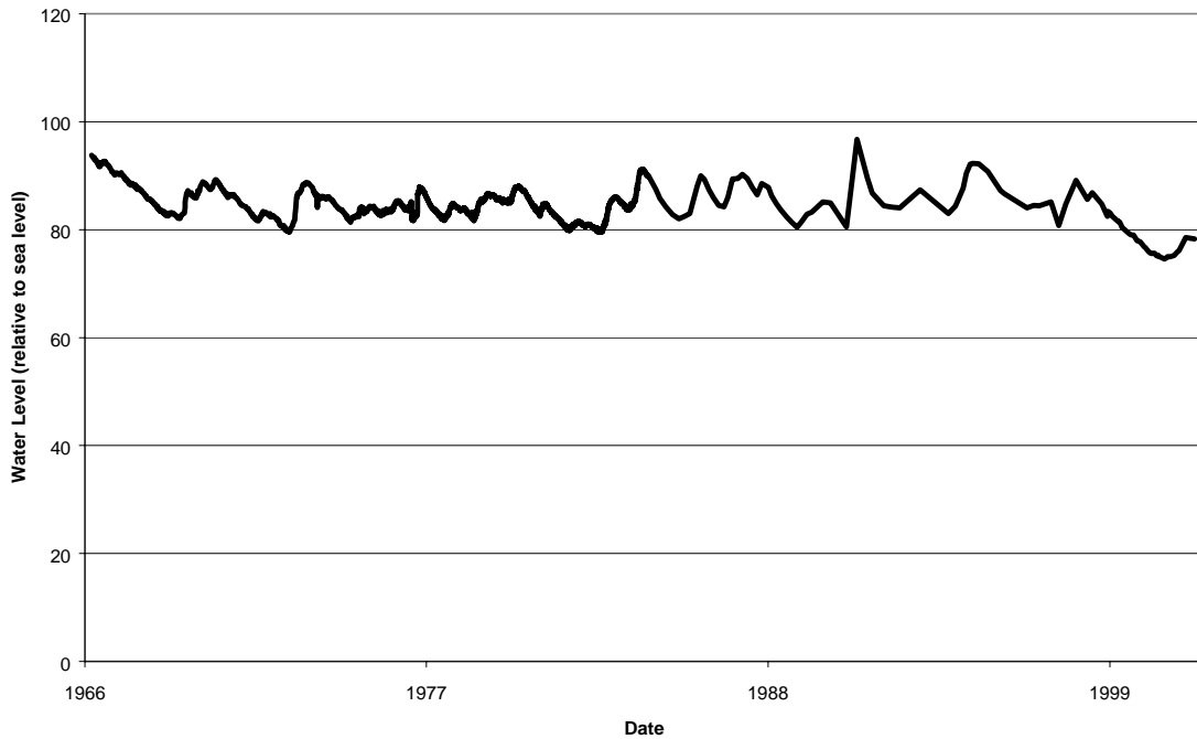
Figure 7. Hydrograph of Lake Jackson Intermediate Aquifer Monitor Well, Northern Leon County. (data from USGS and NFWFMD)
