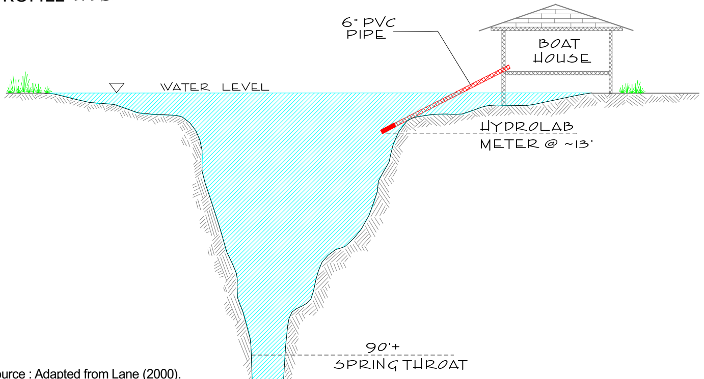
FIGURE 13 CROSS-SECTION OF SPRING CREEK VENT #2 SHOWING HYDROLAB EMBLACEMENT
