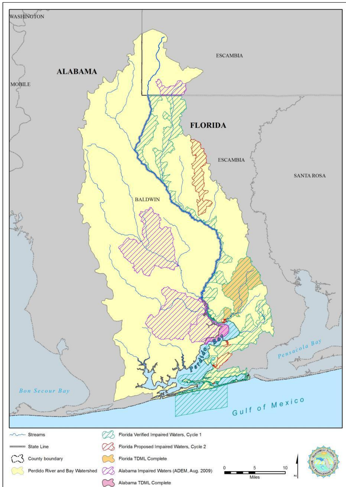
Figure 8. Perdido River and Bay Watershed Impaired Waterbodies
