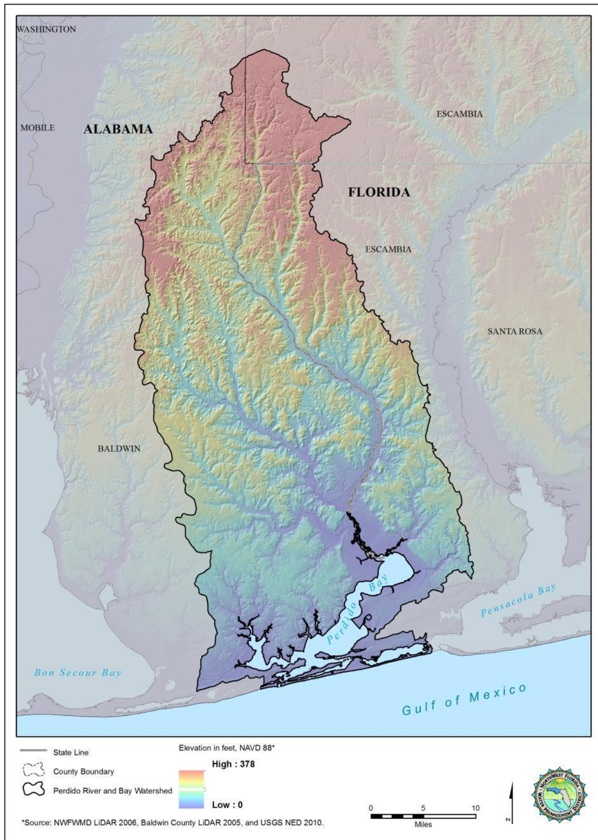
Figure 3. Perdido River and Bay Watershed Topography
