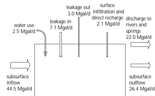
Figure 5-71 Region VI Water Budget for 1991 Calibration Period
