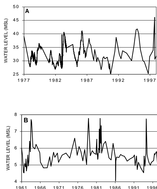
Figure 5-81 Hydrographs of the A) Olson Road and the B) Newport Floridan Aquifer Wells
