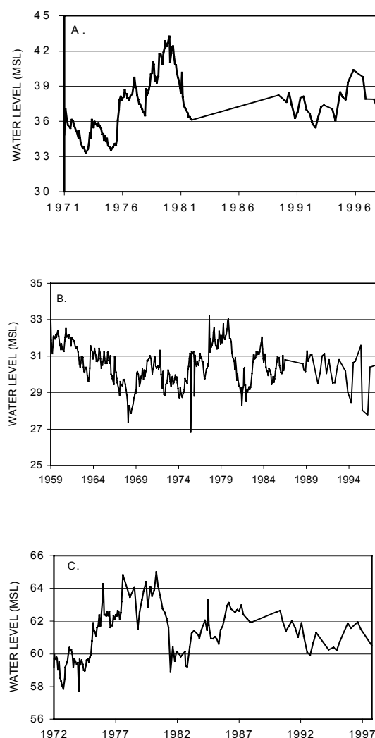
Figure 5-9 Hydrographs of the A) USGS TH2, B) USGS 032-7241A, and C) USGS TH13 Sand-and-Gravel Wells
