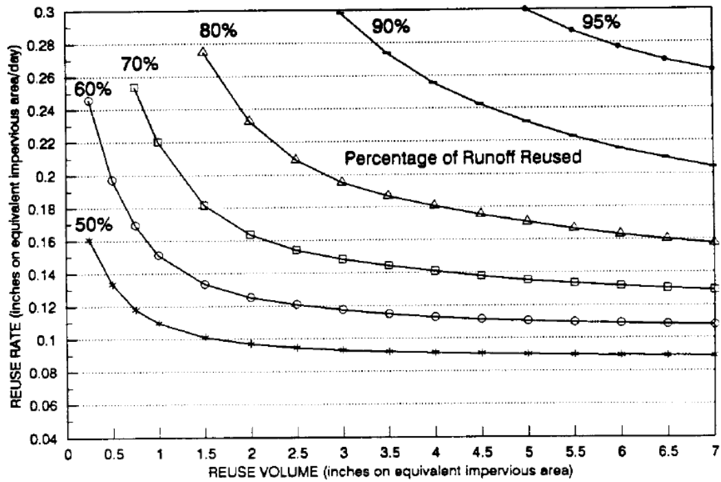
Figure 5-3 Rate-Efficiency-Volume (REV) Curves for Niceville.
