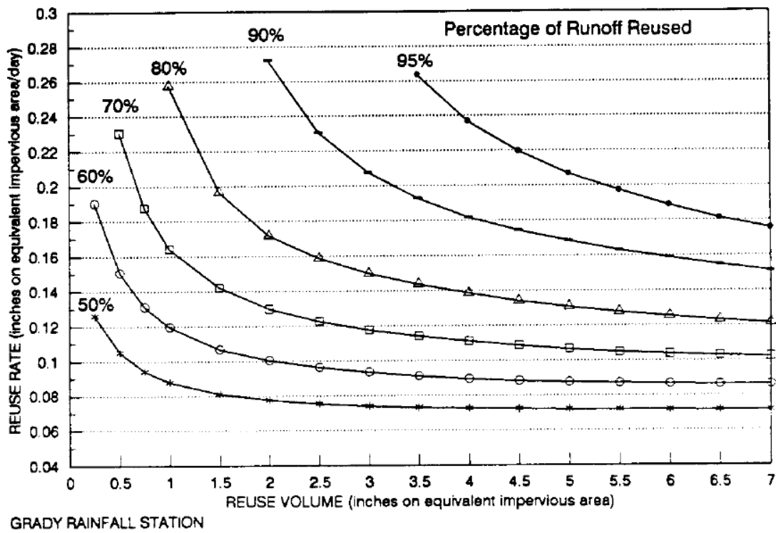
Figure 5-2 Rate-Efficiency-Volume (REV) Curves for Grady.
