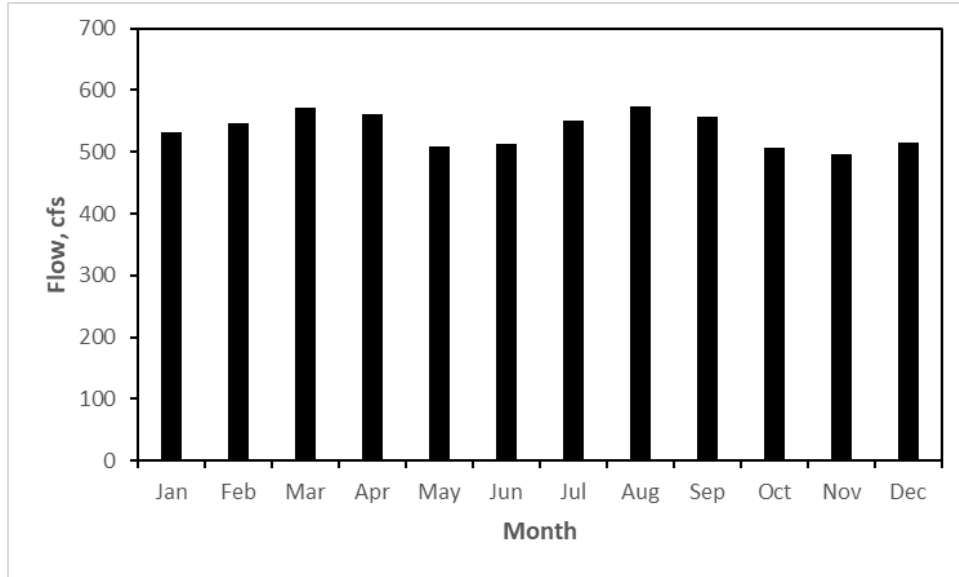
Figure 3-5. Average Monthly Flow at the USGS Station 2359500 Econfina Creek Near Bennett, FL (Econfina Creek @ CR 388)
