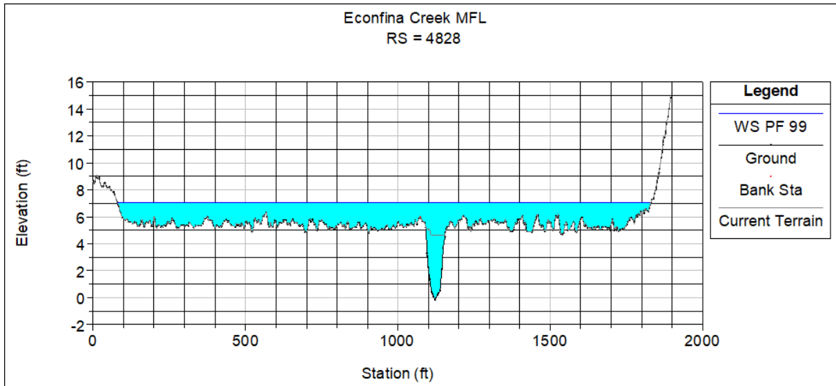
Figure 6-5. Example Model Transect in the Upper and Lower Portion of the Domain. Flows depicted are for the 99 percent percentile A) [text] B) [text]
