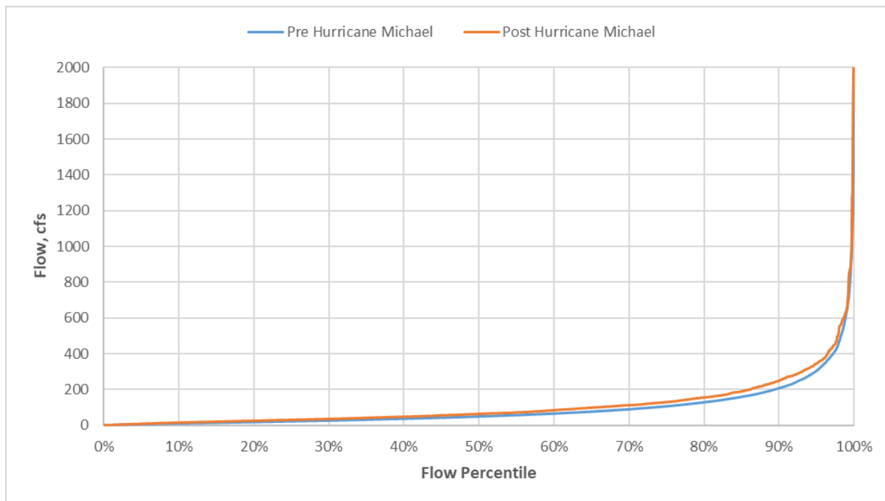
Figure 3-10. Flow Frequency Curve for Surface Water Inputs for the USGS Station 2359500 Econfina Creek Near Bennett, FL (Econfina Creek @ CR 388)
