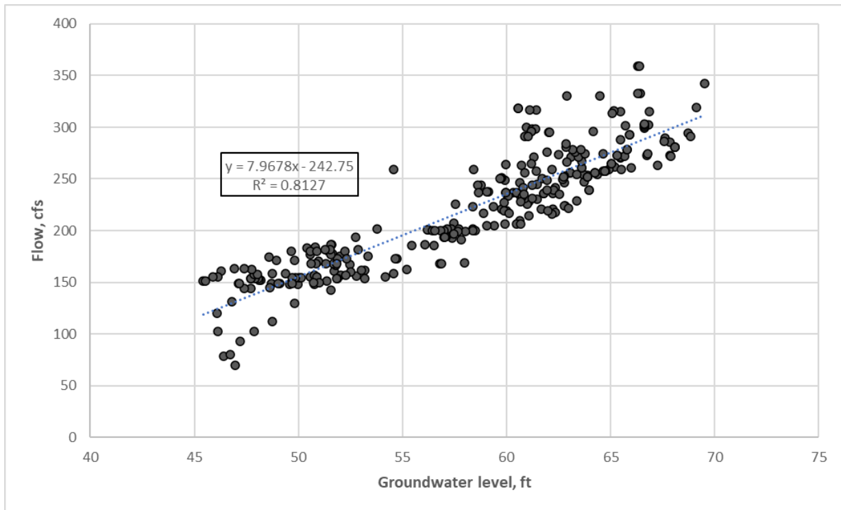
Figure 3-15. Linear Regression Between Baseflow at the NFWFMD Station 8458 Econfina Creek @ SR 20 and Groundwater Level at Greenhead Floridan Monitoring Well (NWFID 3216) from 1998 to 2023
