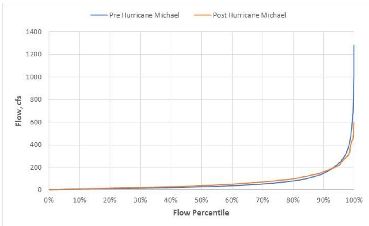
Figure 3-17. Flow Frequency Curve for Surface Water Inputs for the NFWMD Station 8458 Econfina Creek @ SR 20
