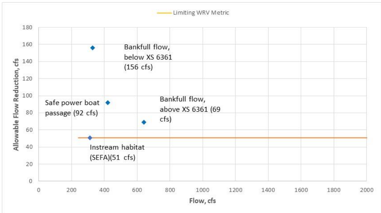
Figure 7-2. Allowable Flow Reductions at Econfinia Creek @ CR 388 for WRV Metrics Evaluated
