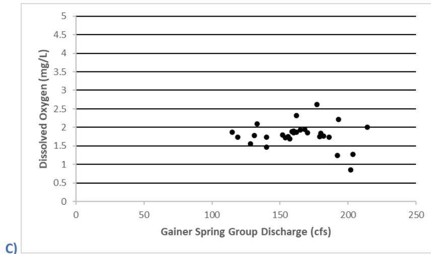
Figure 2-21. A) Nitrate Concentration versus Gainer Spring Group Composite Discharge B) Specific Conductance versus Gainer Spring Group Composite Discharge C) Dissolved Oxygen versus Gainer Spring Group Composite Discharge
