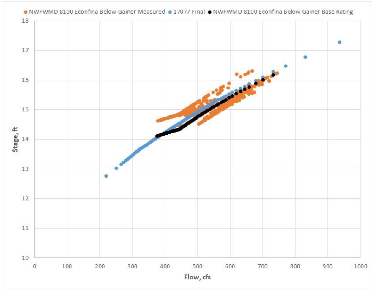
Figure 5-5. Comparison of Measured Stage-Discharge Rating at NFWWMD 8100 (Econfina Creek Below Gainer Spring Group) With Final Simulated Stage-Discharge Rating at XS 17077 (Nearest XS to Econfina Creek Below Gainer Spring Group) for Calibration Period from 4/1/2019 through 9/18/2023
