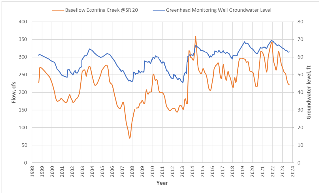
Figure 3-14. Baseflow at the NFWFMD Station 8458 Econfina Creek @ SR 20 versus Groundwater Level at Greenhead Floridan Monitoring Well (NWFID 3216) from 1998 to 2023
