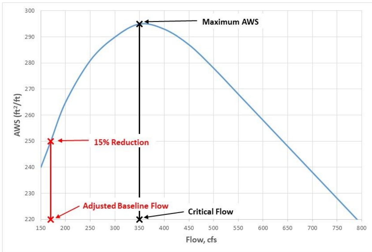
Figure 6-9. Conceptual Depiction of the Estimation of the Critical Flow Resulting in a 15% Reduction in AWS.
