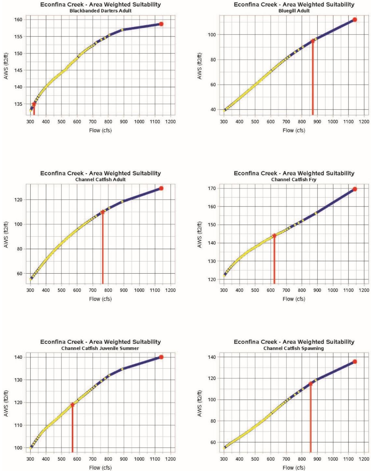
Figure 6-10. Relationship between Flow at Econfina Creek @ CR 388 and AWS for Species and Guilds of Interest.
