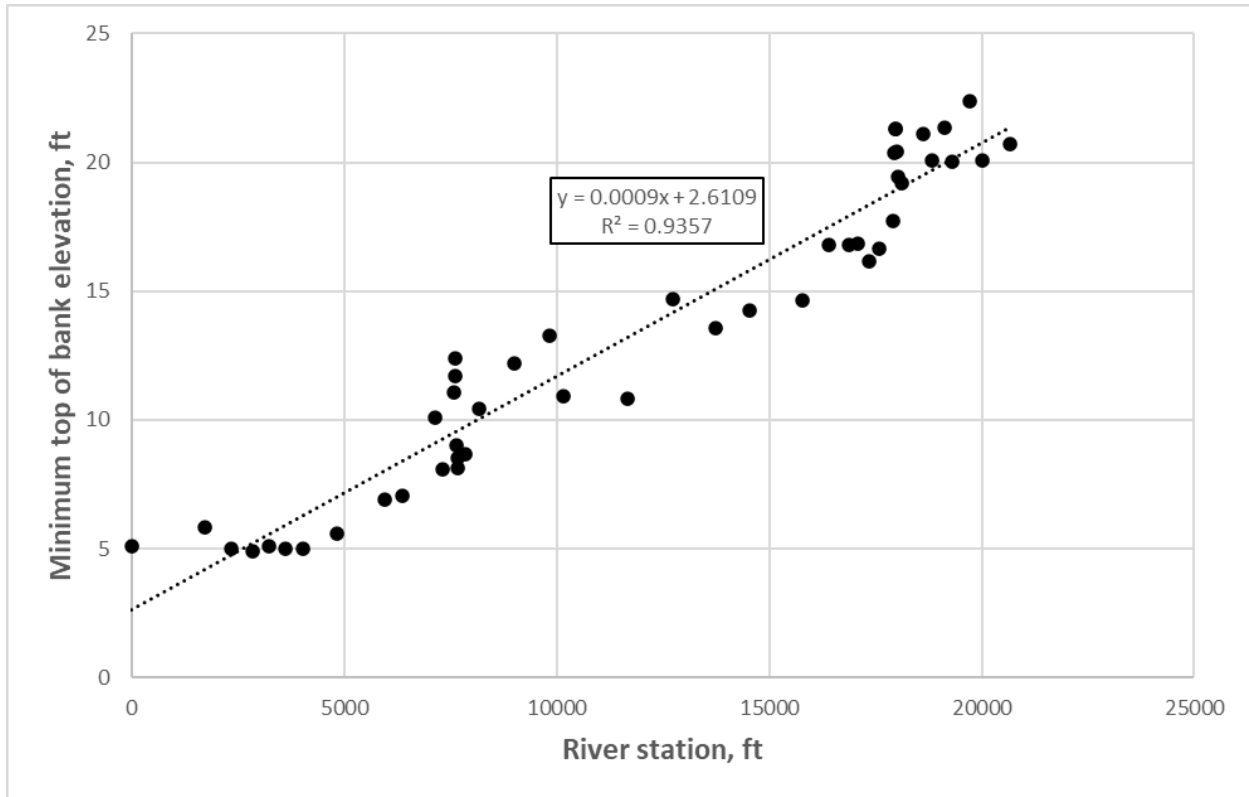
Figure 6-8. Bank Profile for Econfina Creek Study Area
