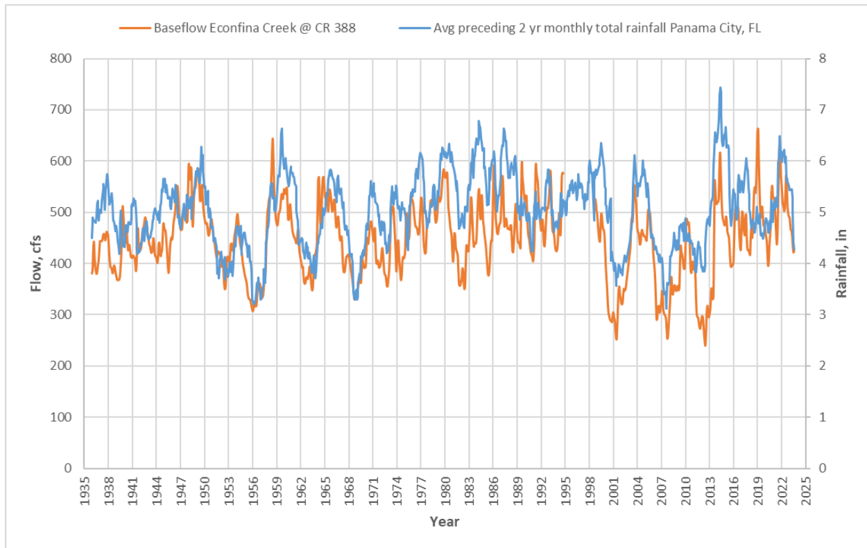
Figure 3-6. Baseflow at the USGS Station 2359500 Econfina Creek Near Bennett, FL (Econfina Creek @ CR 388) versus Preceding Two-year Moving Average Monthly Total Rainfall from the National Weather Service Station USC00086842 Located in Panama City, Florida
