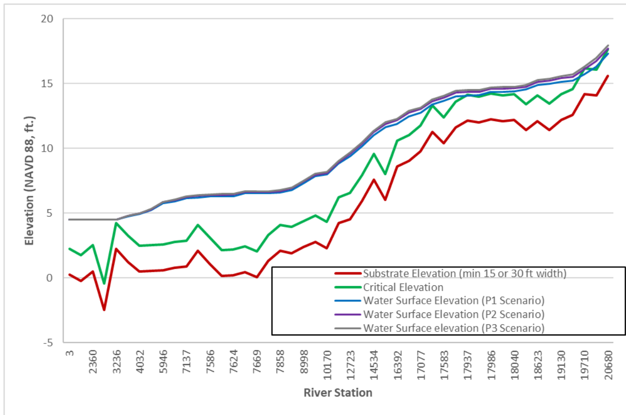
Figure 6-2. Critical Elevation and Minimum Modeled Water Levels for Safe Power Boat Passage Along Econfina Creek
