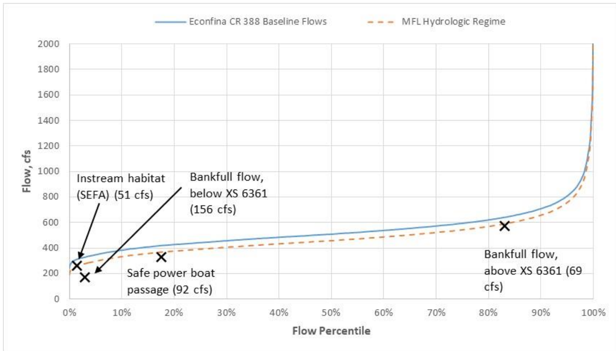
Figure 7-1. Proposed MFL Flow Frequency Curve for Econfinia Creek @ CR 388 for WRV Metrics Evaluated
