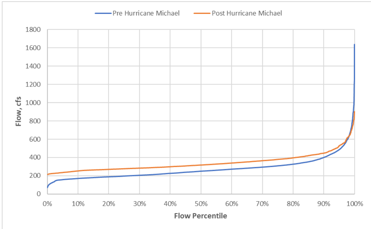
Figure 3-16. Flow Frequency Curve for the NFWMD Station 8458 Econfina Creek @ SR 20
