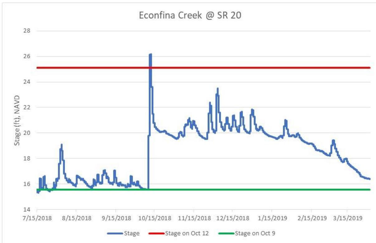
Figure 2-23. Econfina Creek Stage @ SR 20 from 7/15/2018 to 4/1/2019.
