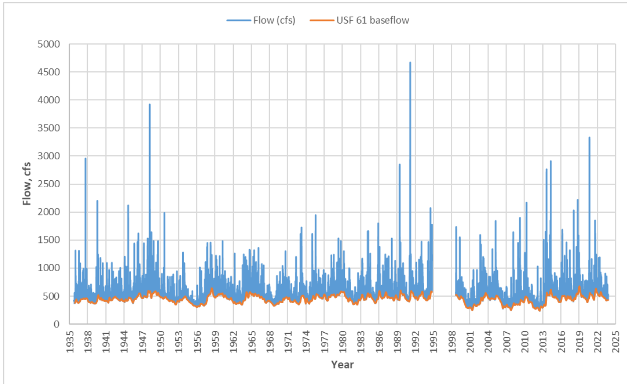
Figure 3-4. Daily Flow Hydrograph and Baseflow Hydrograph at the USGS Station 2359500 Econfina Creek Near Bennett, FL (Econfina Creek @ CR 388)
