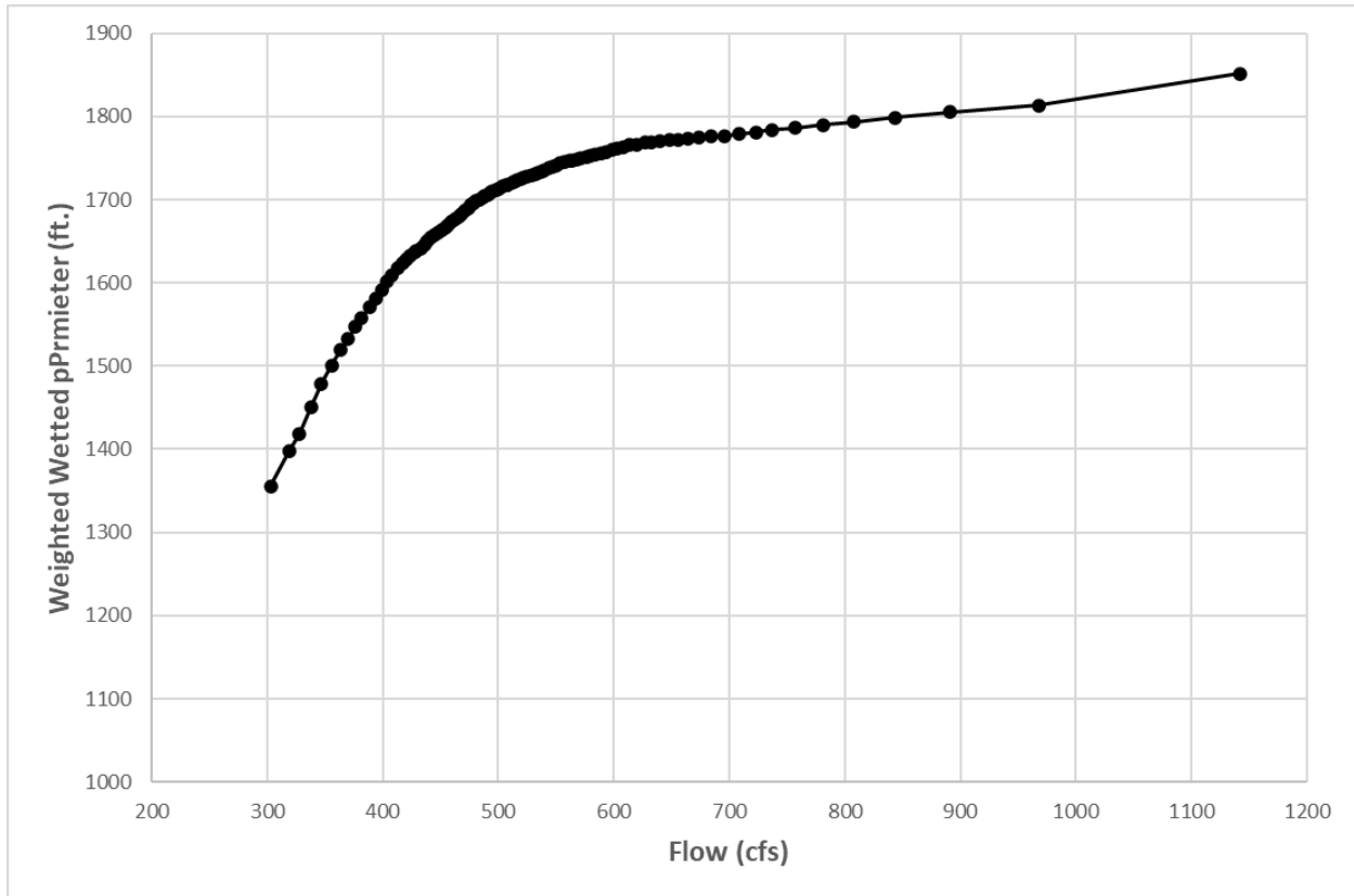
Figure 6-7. Average Transect Weighted Wetted Perimeter versus Flow at Econfina Creek @ SR 20 below XS 6361
