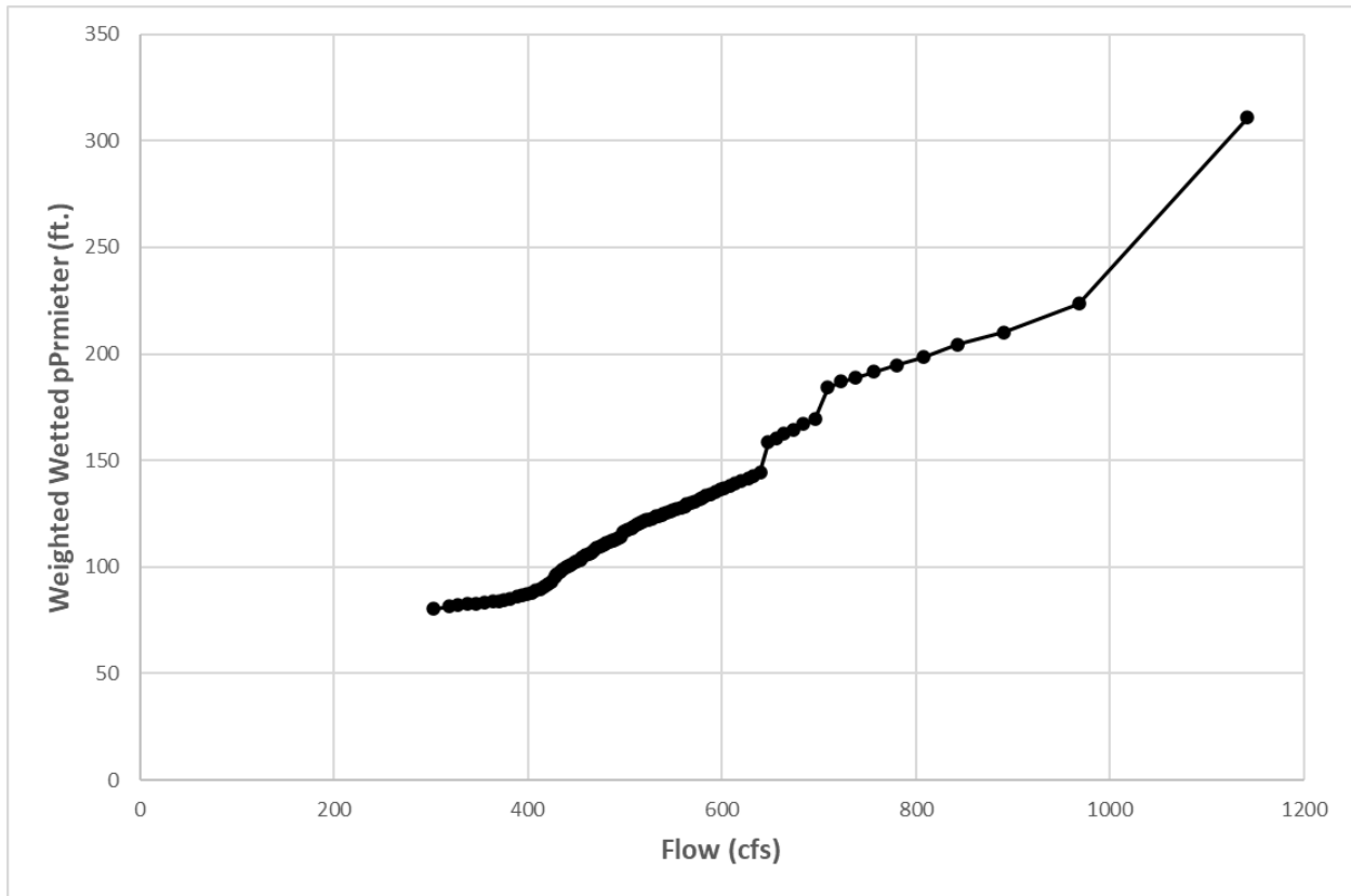
Figure 6-6. Average Transect Weighted Wetted Perimeter versus Flow at Econfina Creek @ CR 388, above XS 6361
