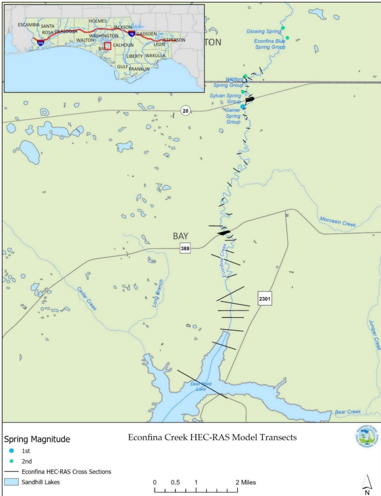
Figure 5-1. Econfina Creek and Springs MFL HEC-RAS Model Extent
