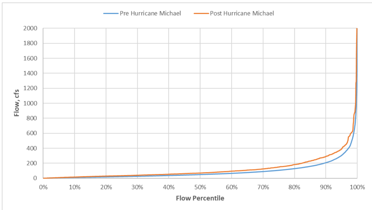
Figure 2-8. Flow Frequency Curve for Surface Water Inputs for the USGS station 2359500 Econfina Creek Near Bennett, FL (Econfina Creek @ CR 388)
