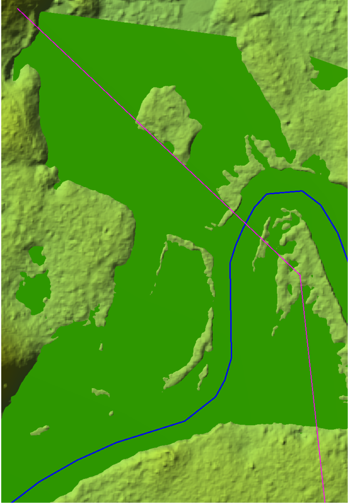
Figure 2-12. RS 19319, 99th percentile flows
