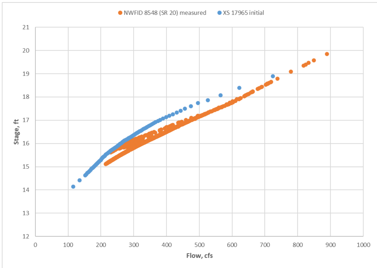
Figure 3-3. Comparison of measured stage-discharge rating at NWFMD 8548 (Econfina Creek @ SR 20) with Initial simulated stage-discharge rating at XS 17965 (nearest XS to Econfina Creek @ SR 20 station)
