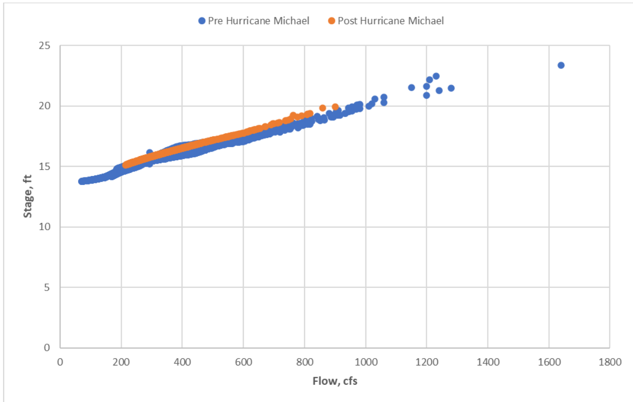
Figure 3-2. Comparison of stage-discharge relationships for the NFWWMD station 8458 Econfina Creek @ SR 20
