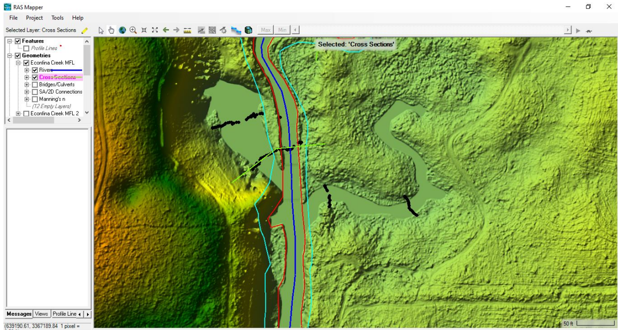
Figure 2-4. Digitization of Cross Sections overlaying survey points in RAS Mapper
