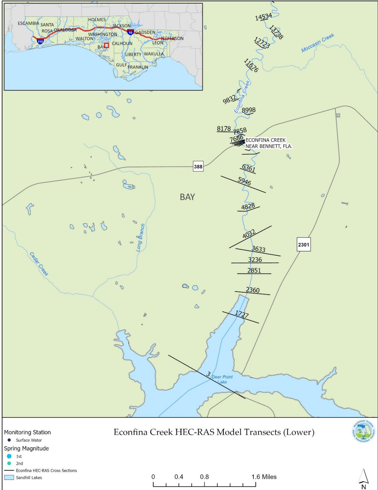
Figure 5-1 C) Econfina Creek and Spring MFL HEC-RAS Model Extent – Lower Creek
