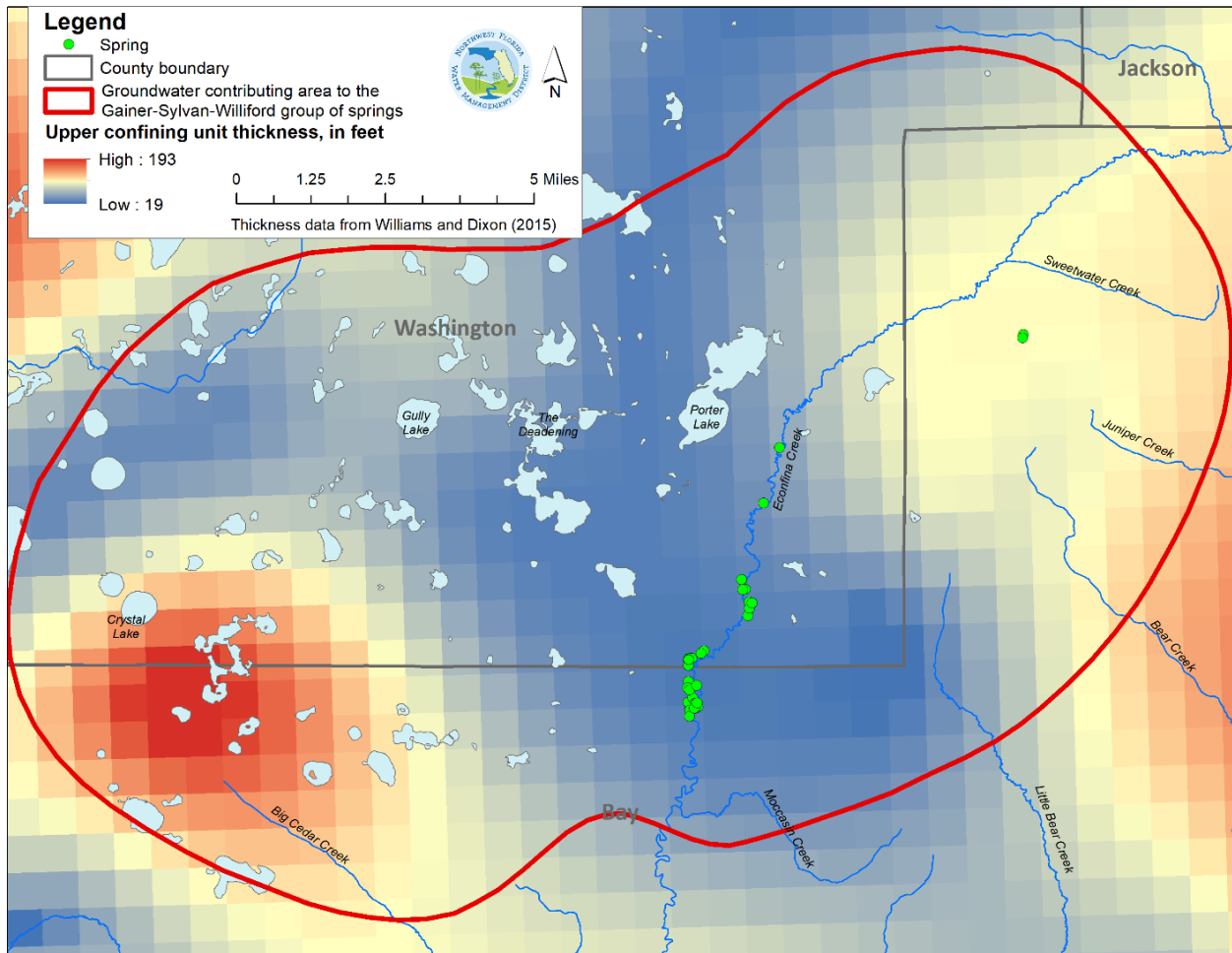
Figure 2-11. Estimated Thickness of the Upper Confining Unit of the Floridan Aquifer System in the Vicinity of the Contributing Area to the Middle Reach of Econfina Creek and Associated Springs, Based on Data From Williams And Dixon (2015)
