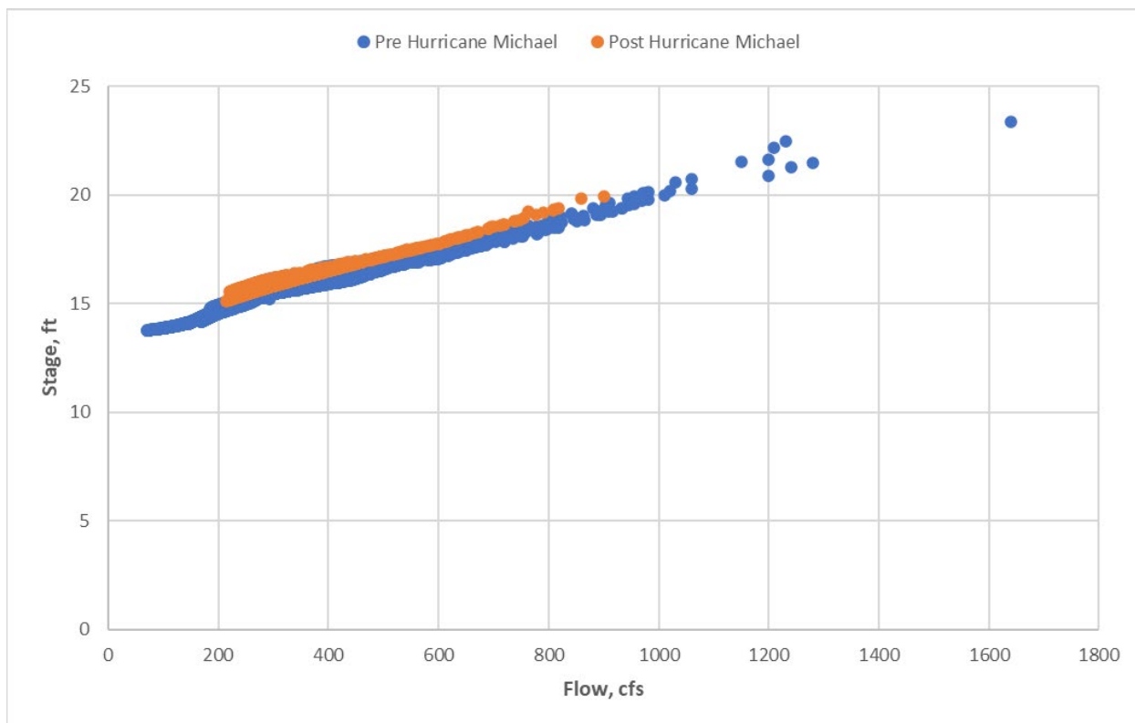
Figure 3-18. Comparison of Stage-Discharge Relationships for the NFWFMD Station 8458 Econfina Creek @ SR 20
