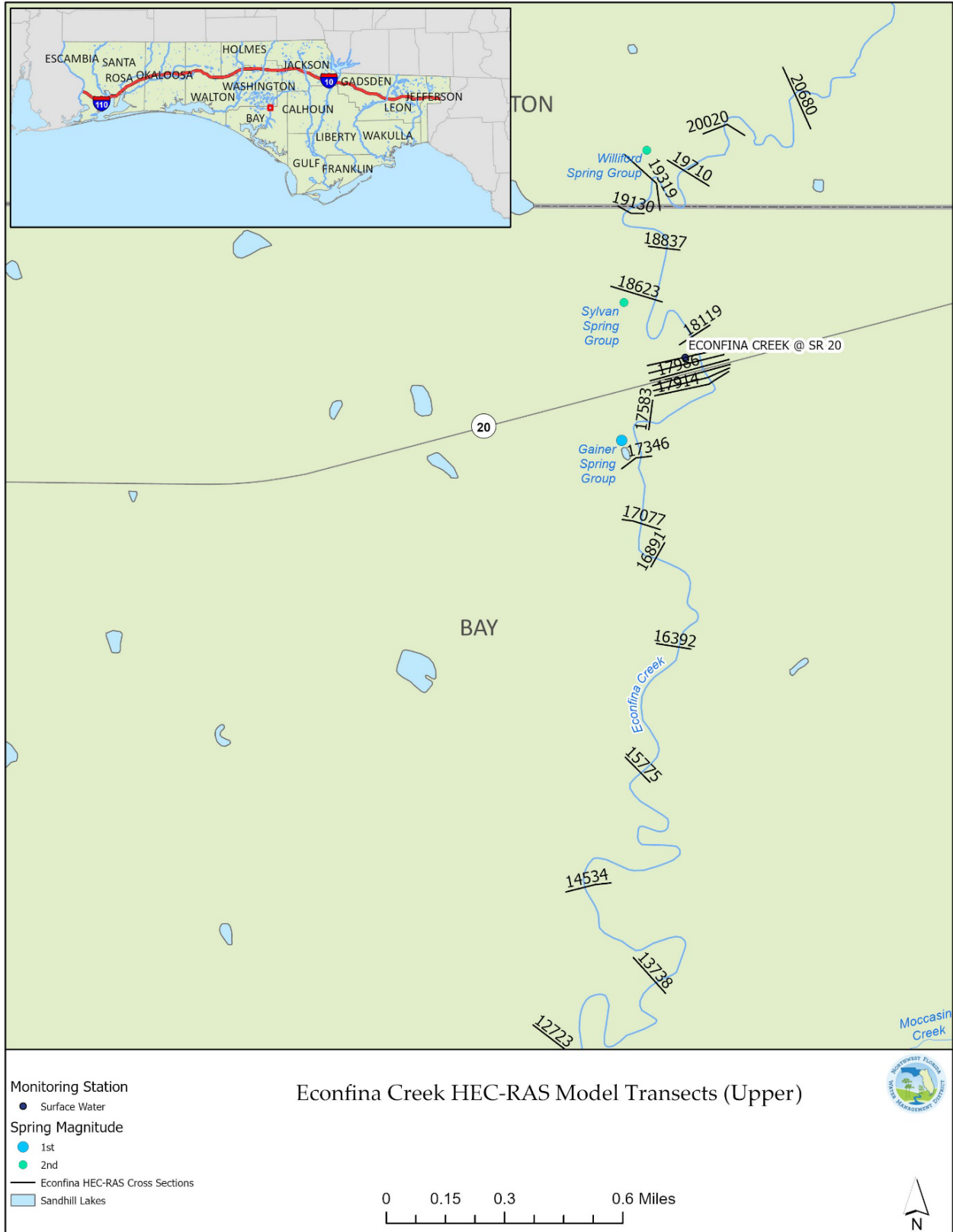
Figure 5-1 B) Econfinia Creek and Sprins MFL HEC-RAS Model Extent – Upper Creek
