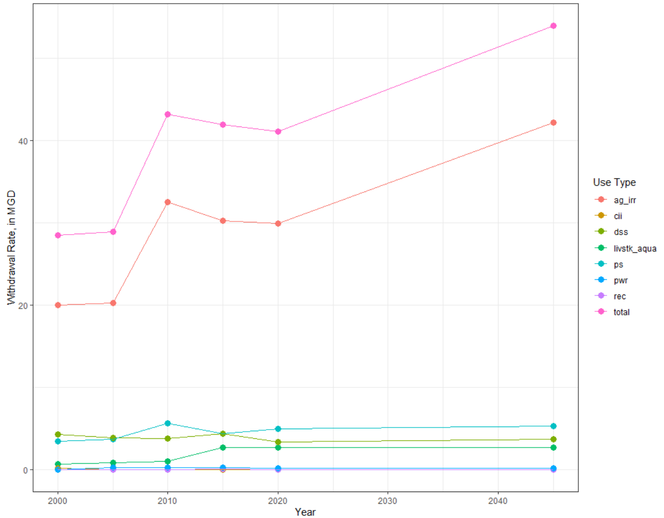
Figure 4-30. NCDM groundwater withdrawal estimates for selected years by water-use type (agg_irr, agricultural irrigation; cii, commercial-industrial-institutional; dss, domestic self-supply; livstk_aqua, livestock and aquaculture; ps, public supply; pwr, power generation; rec, recreational; total, total use across all use types).
