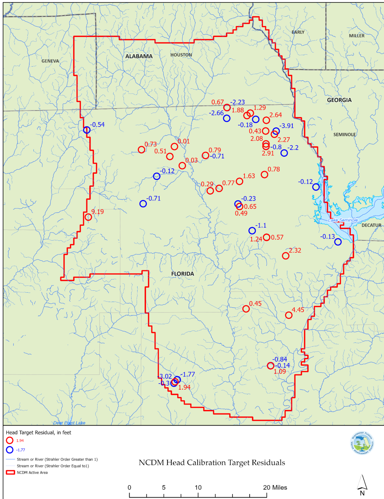
Figure 6-4. Map of differences (residuals) between simulated and calibration target values of groundwater levels.
