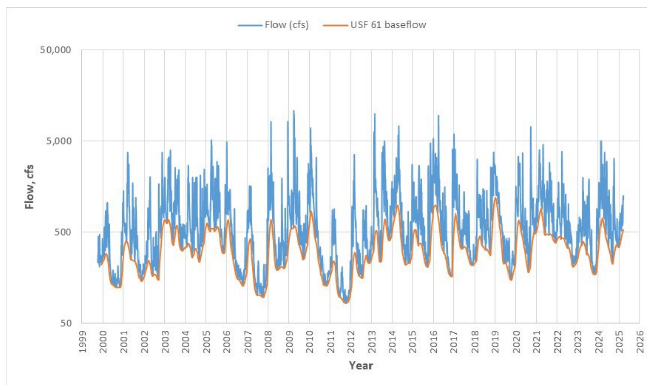
Figure 4-17. Daily flow hydrograph and baseflow hydrograph at the USGS Station 2358789 Chipola River near Marianna, FL.
