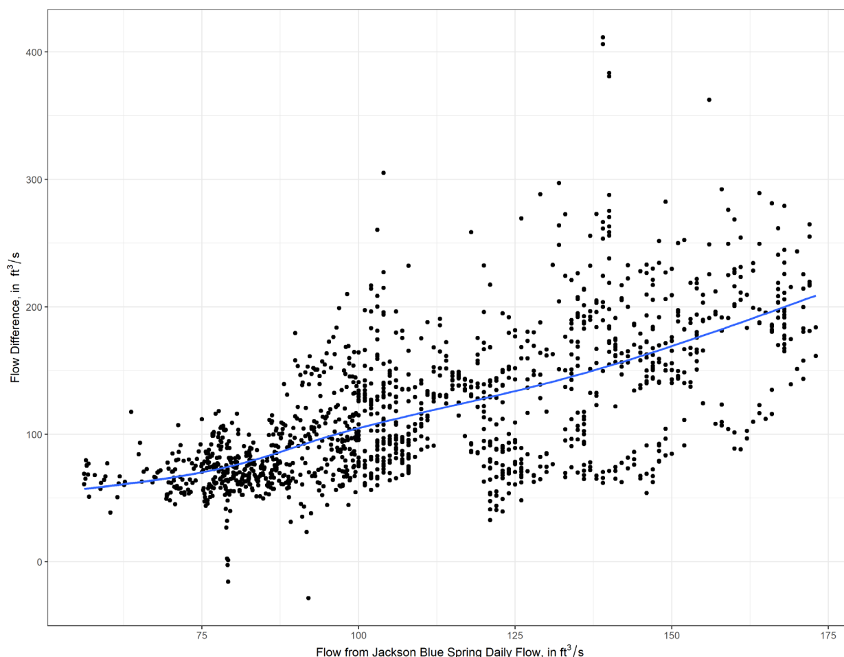
Figure 4-25. Scatterplot with LOESS regression fit of daily mean Merritts Mill Pond pickup versus concurrent daily mean Jackson Blue Spring flows
