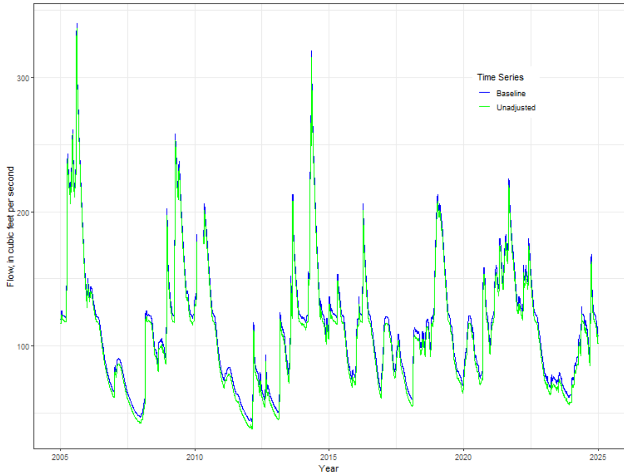
Figure 7-2. Time-series plot of baseline and unadjusted lateral inflows to Merritts Mill Pond.
