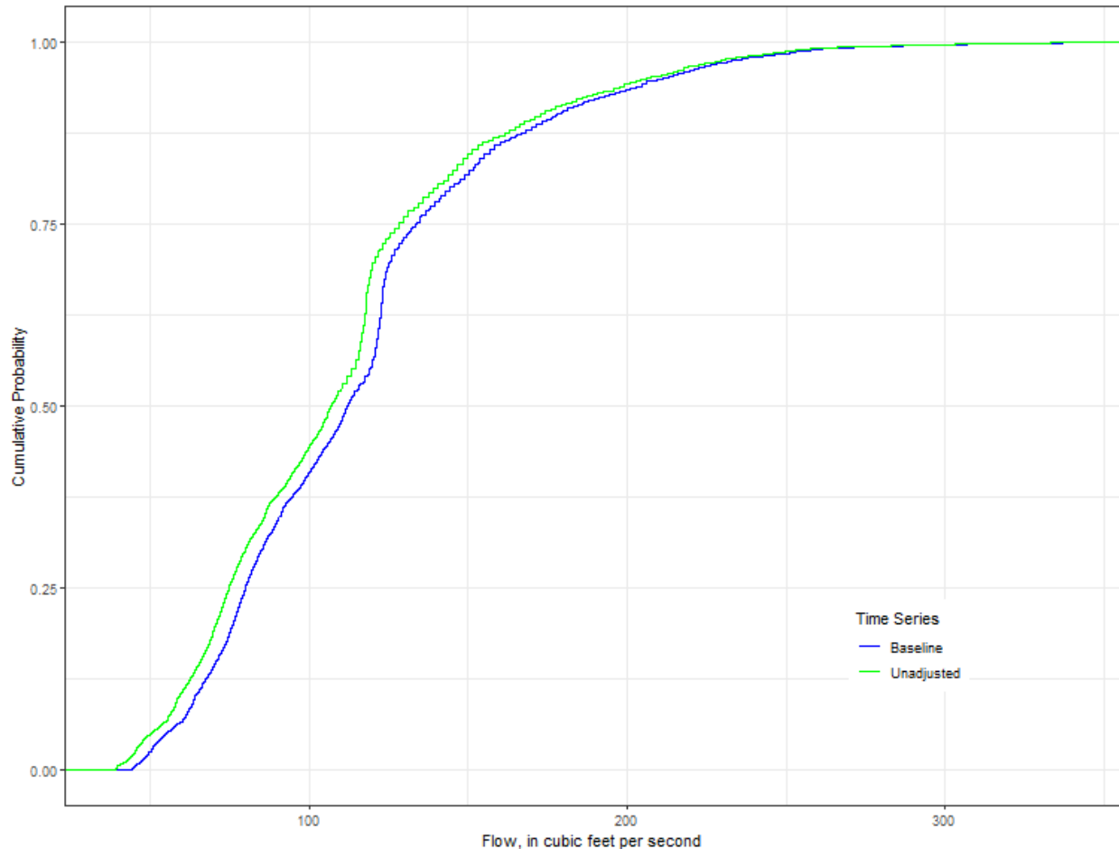
Figure 7-4. Cumulative probability plots of daily values from unadjusted and baseline time series of lateral inflows to Merritts Mill Pond.
