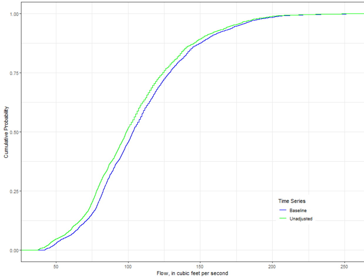
Figure 7-3. Cumulative probability plots of daily values from unadjusted and baseline time series of Jackson Blue Spring flows.
