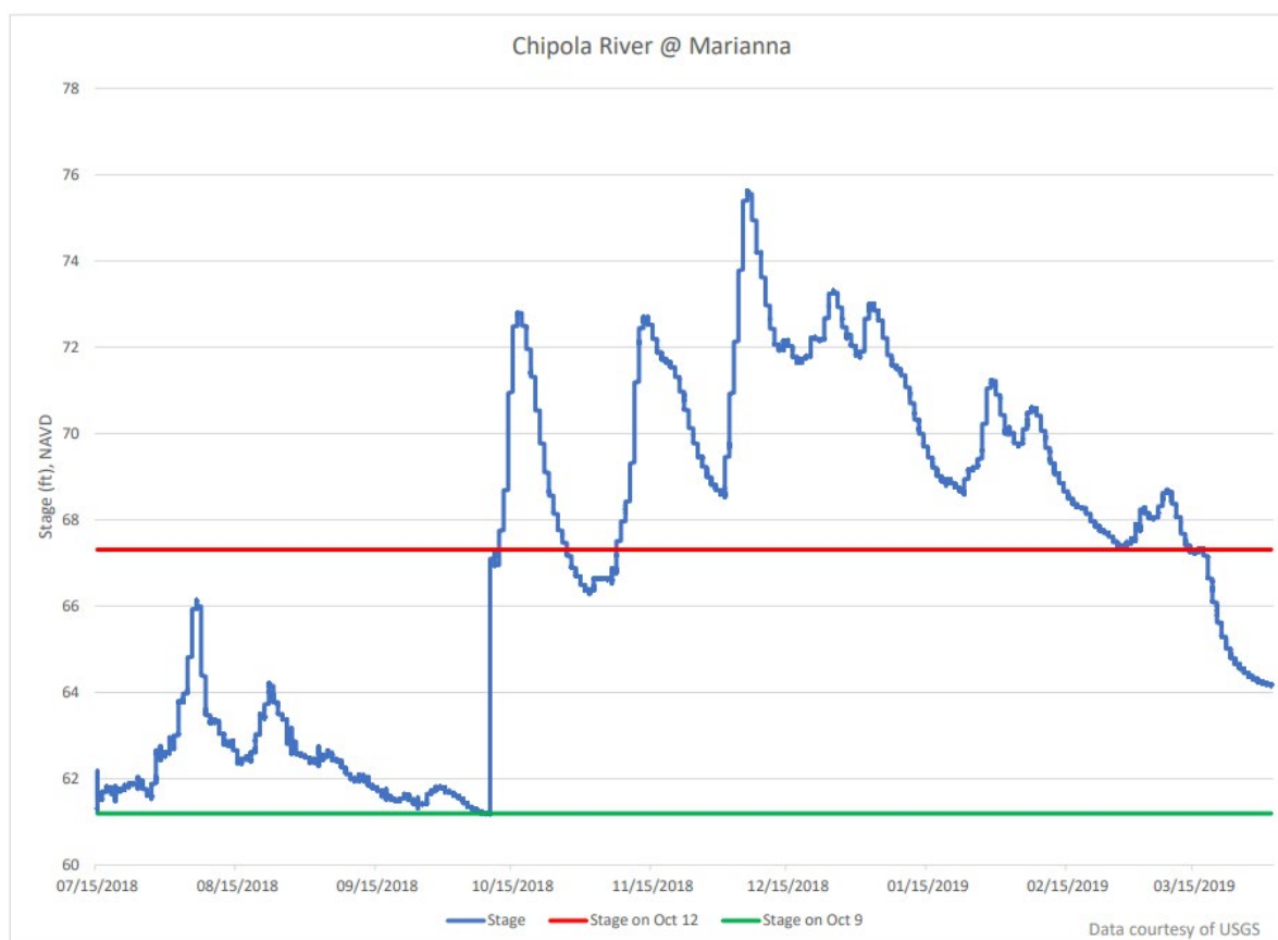
Figure 4-5. Chipola River Stage at USGS 02358789 Chipola River at Marianna from July 15, 2018 to April 1, 2019.
