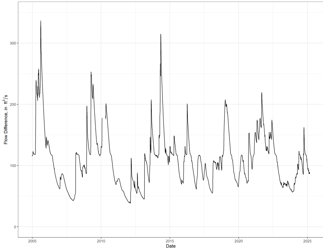
Figure 4-26. Time series of estimated daily Merritts Mill Pond flow difference (pickup) values for the period from January 1, 2005 through December 31, 2024.
