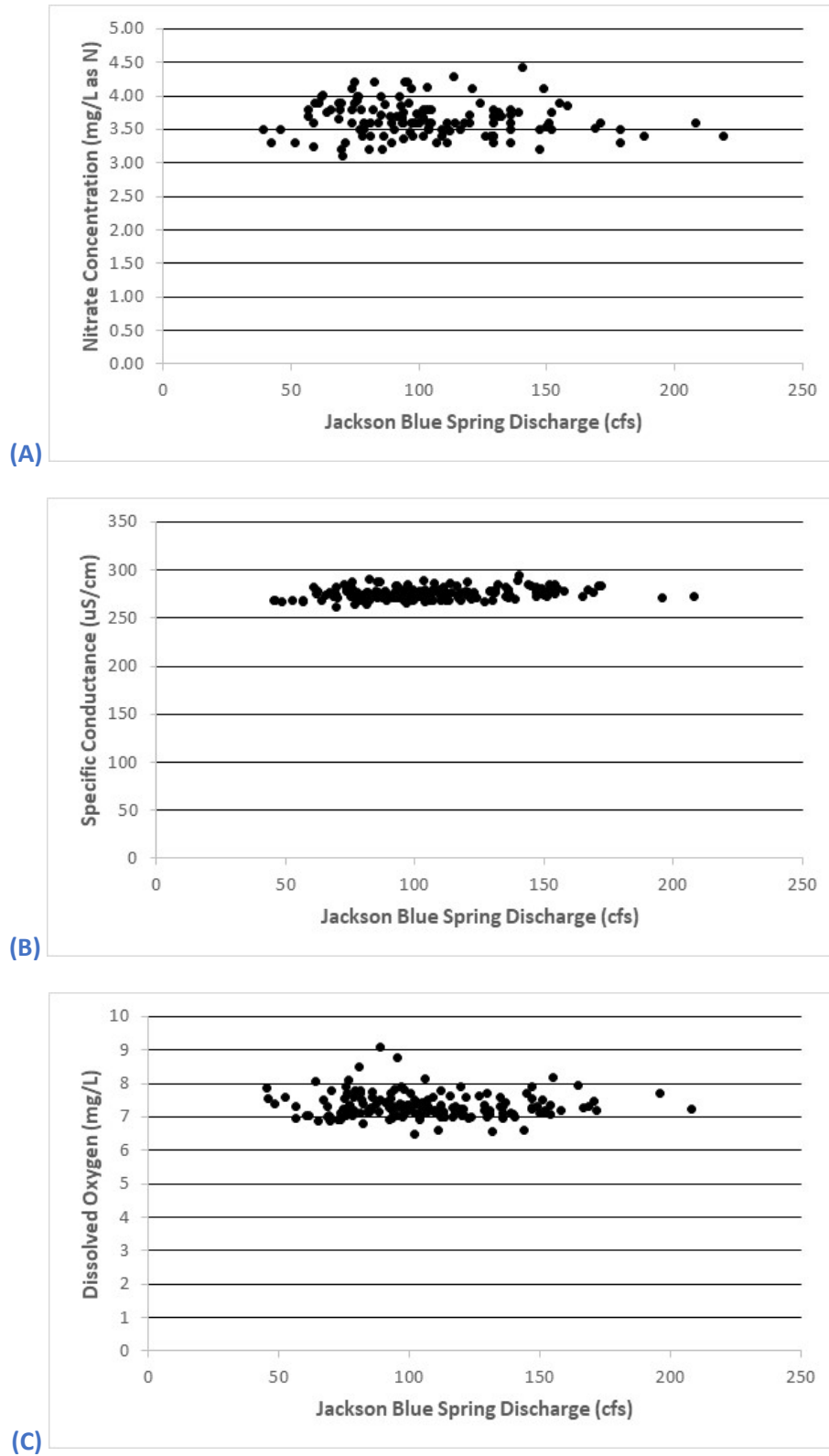
Figure 3-2. (A) Nitrate concentration versus Jackson Blue Spring Discharge (B) specific conductance versus Jackson Blue Spring Discharge, and (C) Dissolved oxygen versus Jackson Blue Spring discharge.
