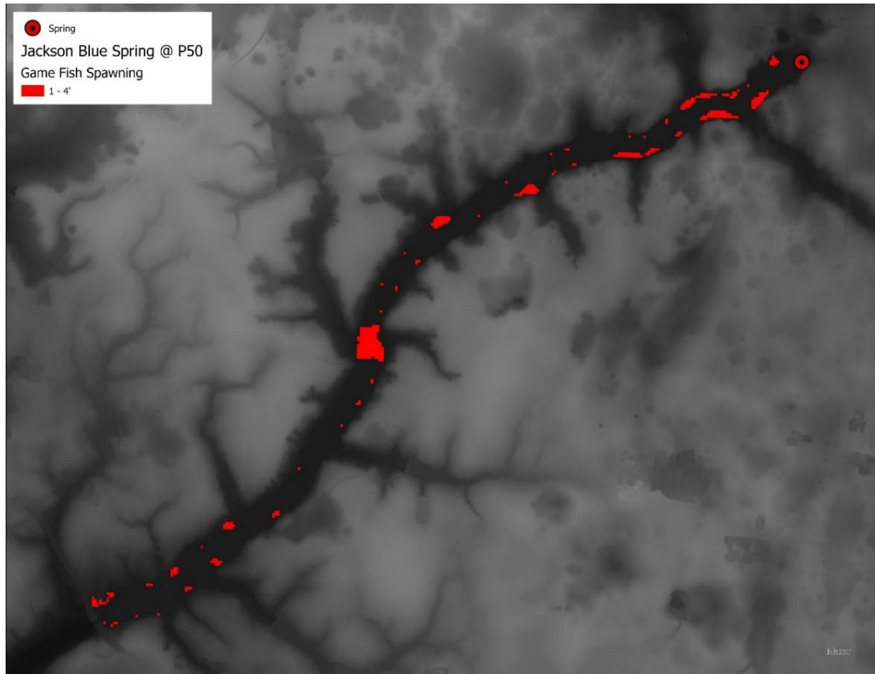
Figure 7-15. Areas within the game fish spawning critical depth range at the median baseline flow.
