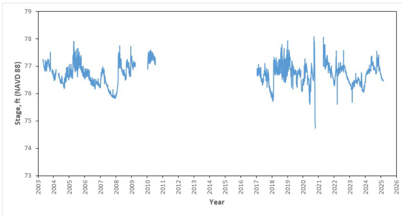
Figure 4-27. Daily average stage at USGS 2358795 Jackson Blue Spring near Marianna.
