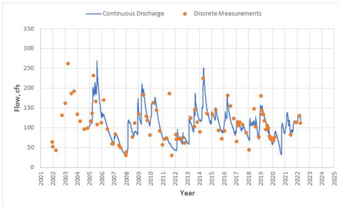
Figure 4-10. Continuous daily average and discrete discharge measurements at Jackson Blue Spring (2001 - 2024).
