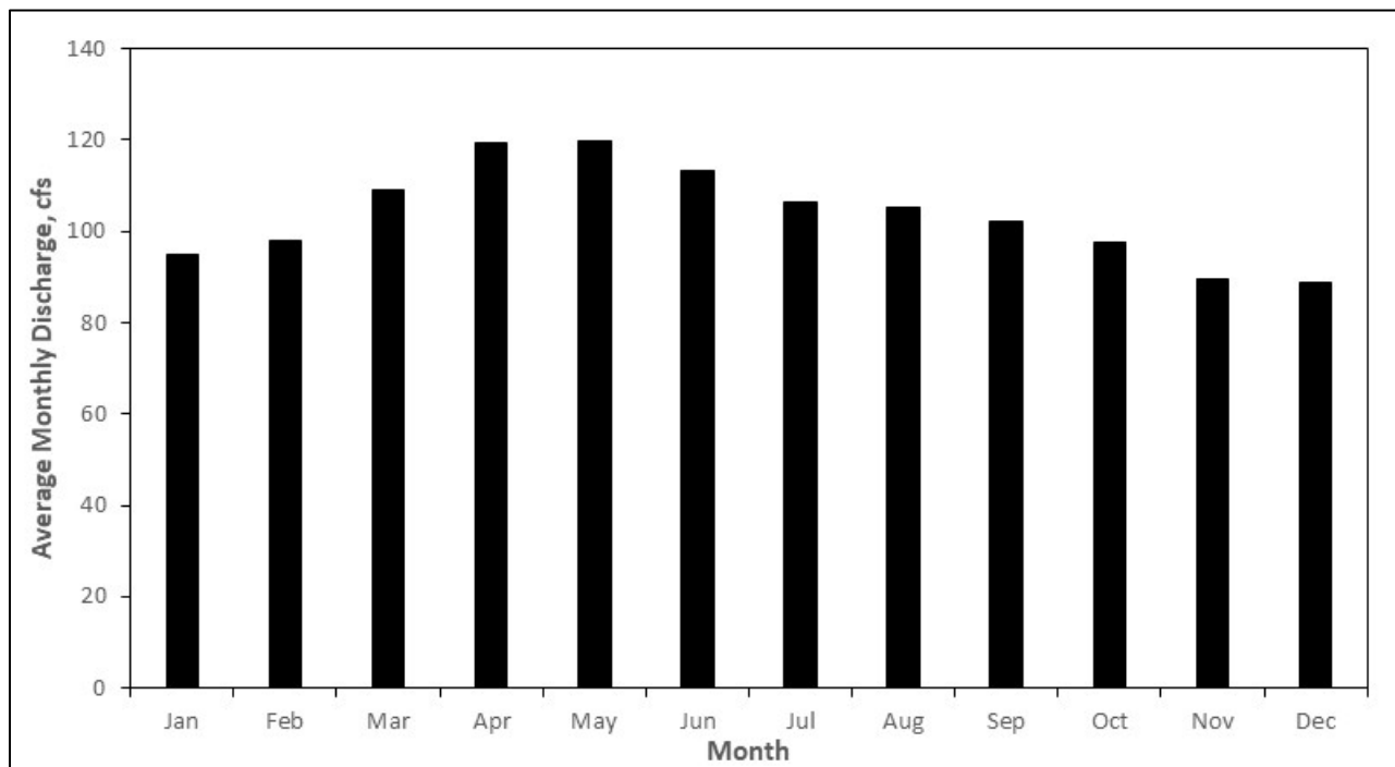
Figure 4-12. Average Monthly Jackson Blue Spring discharge.
