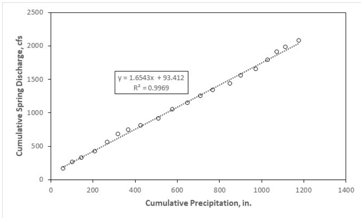
Figure 4-16. Double mass curve between cumulative precipitation at NWS Chipley, FL and cumulative Jackson Blue Spring discharge
