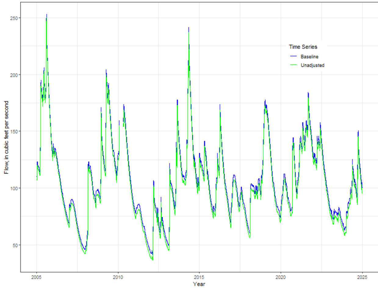
Figure 7-1. Time-series plot of baseline and unadjusted Jackson Blue Spring flows.
