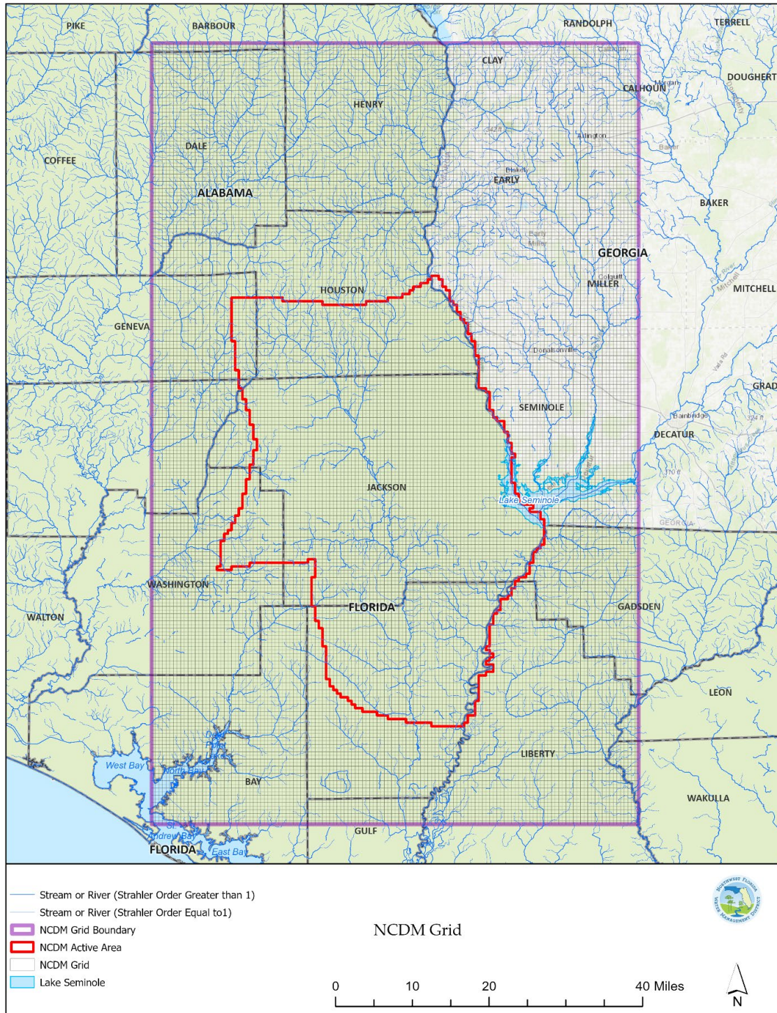
Figure 6-2. NCDM model grid.
