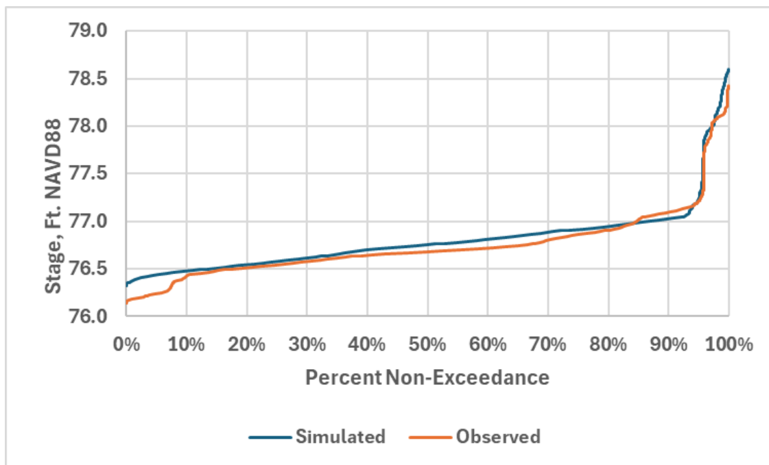
Figure 6-10. Stage duration curves for the calibration simulation, comparing observed and simulated stages at the US 90 Bridge on Merritts Mill Pond.
