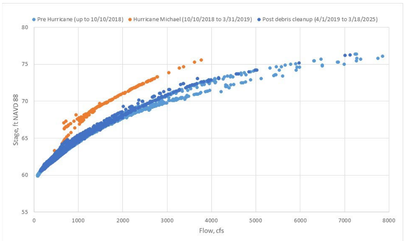
Figure 4-21. Comparison of stage-discharge relationships for the USGS station 02358789 Chipola River at Marianna.
