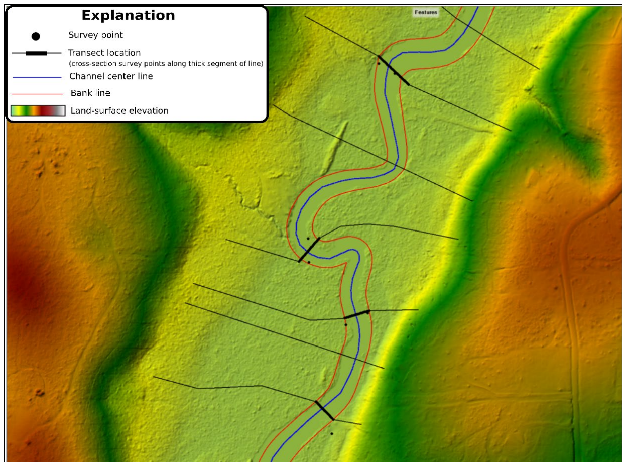
Figure 6-8. Digitization of cross sections overlaying survey points in RAS Mapper.
