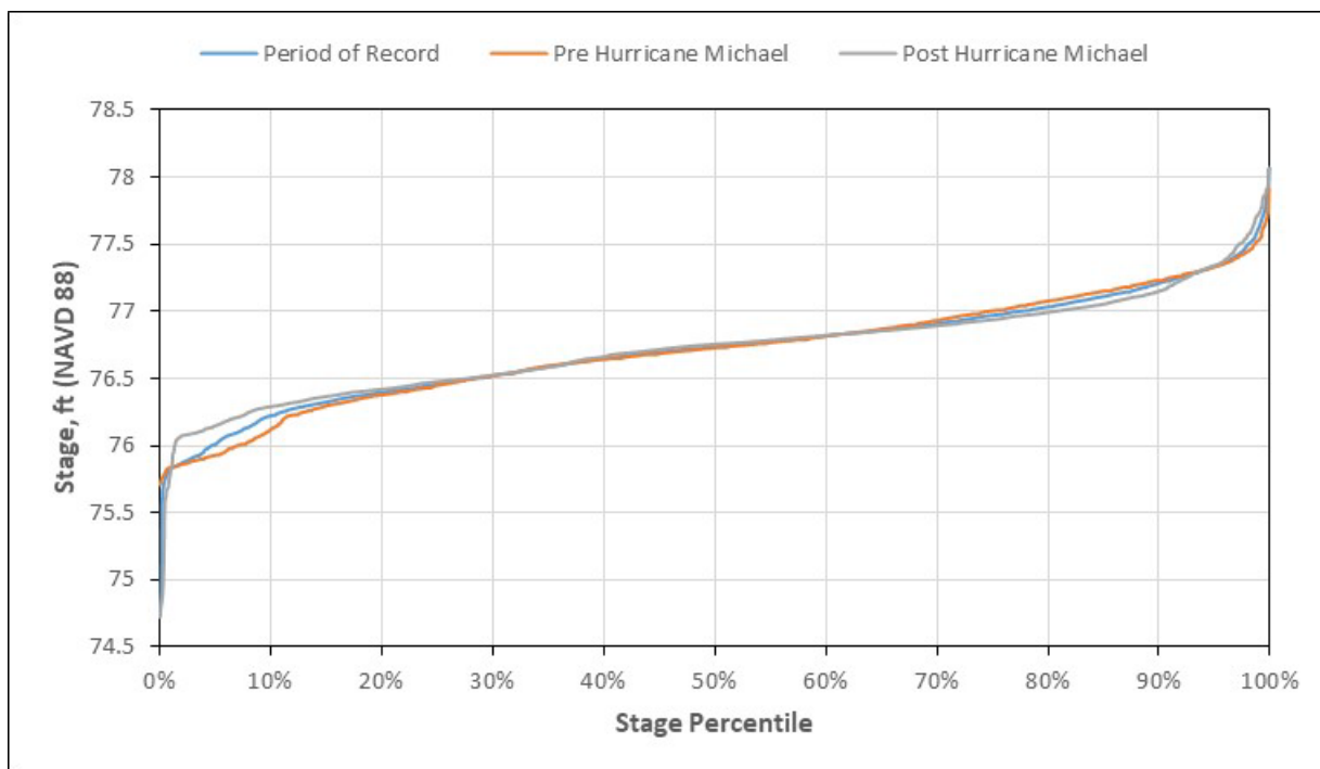
Figure 4-28. Stage duration curves at USGS 2358795 Jackson Blue Spring near Marianna.
