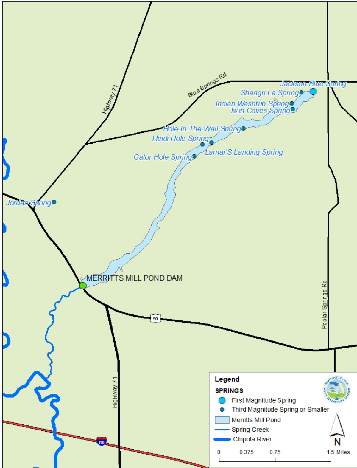
Figure 2-4. Locations of springs along Merritts Mill Pond and Spring Creek and Merritts Mill Pond dam.
