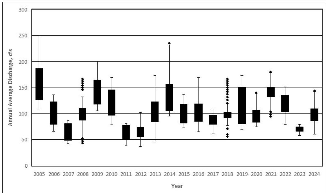
Figure 4-11. Boxplot of Jackson Blue Spring discharge.
