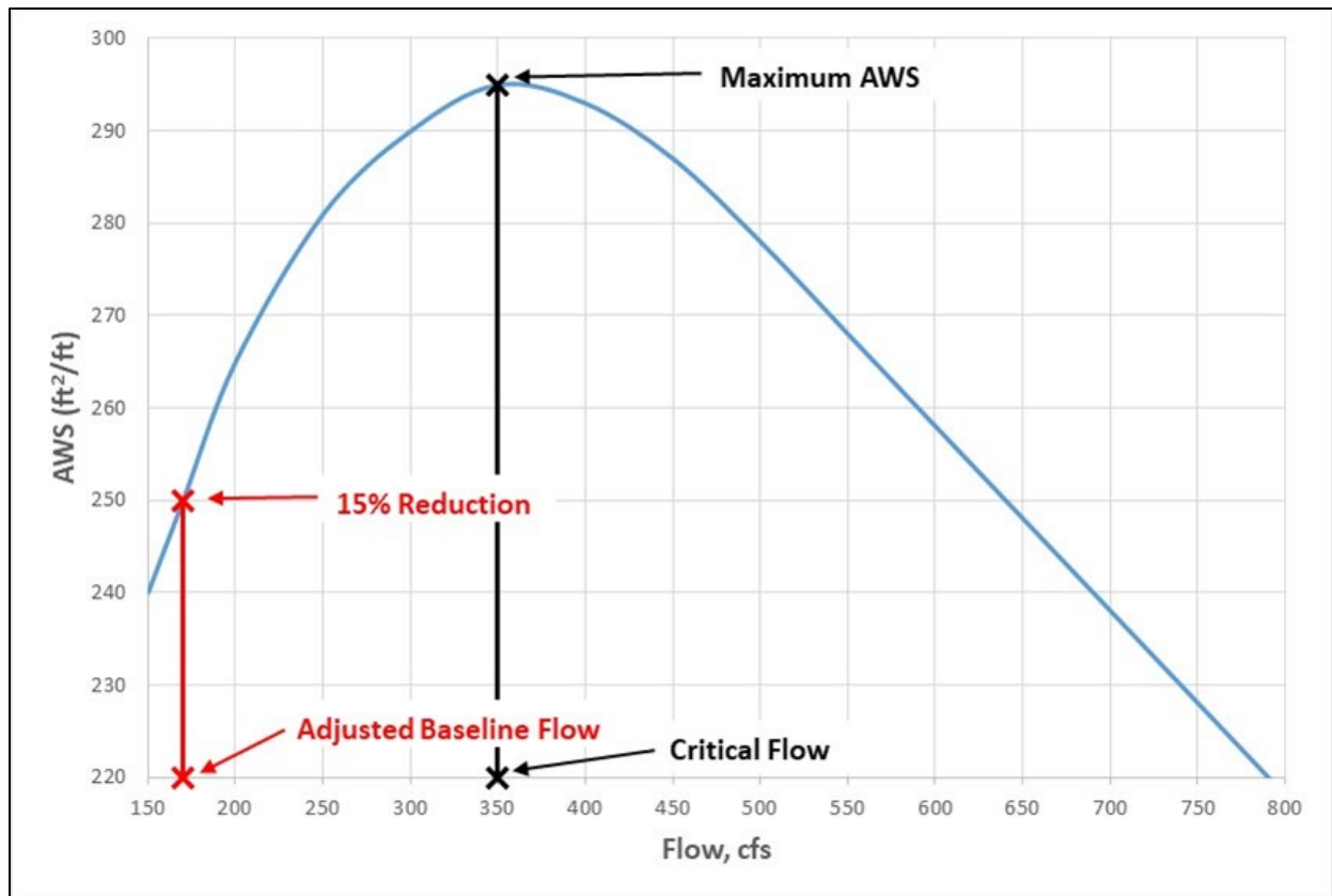
Figure 7-10. Conceptual diagram of the estimation of the critical flow resulting from a 15-percent reduction in Area Weighted Suitability (AWS).
