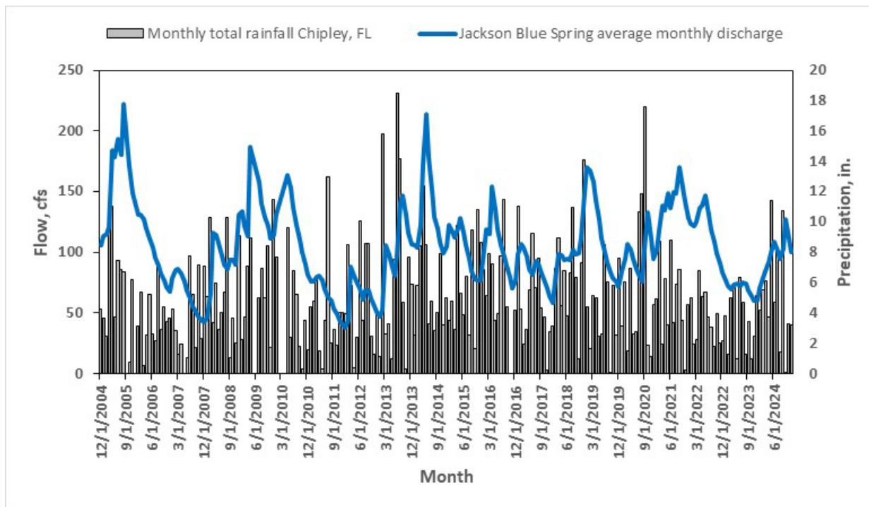
Figure 4-13. Comparison of monthly total rainfall at NWS Chipley, FL and Jackson Blue Spring average monthly discharge.
