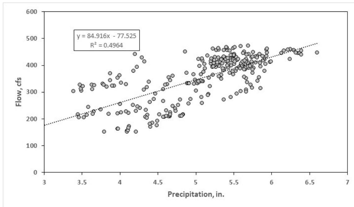
Figure 4-19. Linear Regression between preceding 2 year moving average monthly total rainfall from the National Weather Service station USC00081544 located in Chipley, Florida and 4-month lagged, 2-year moving average baseflow at the USGS Station 2358789 Chipola River Near Marianna, FL
