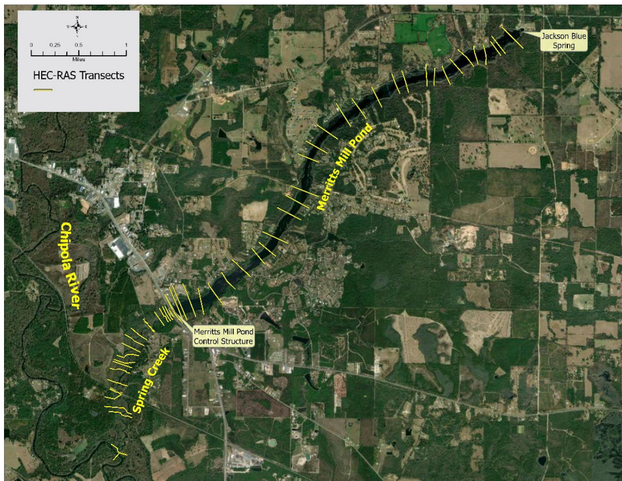
Figure 7-12. Transect locations in Merritts Mill Pond and Spring Creek.
