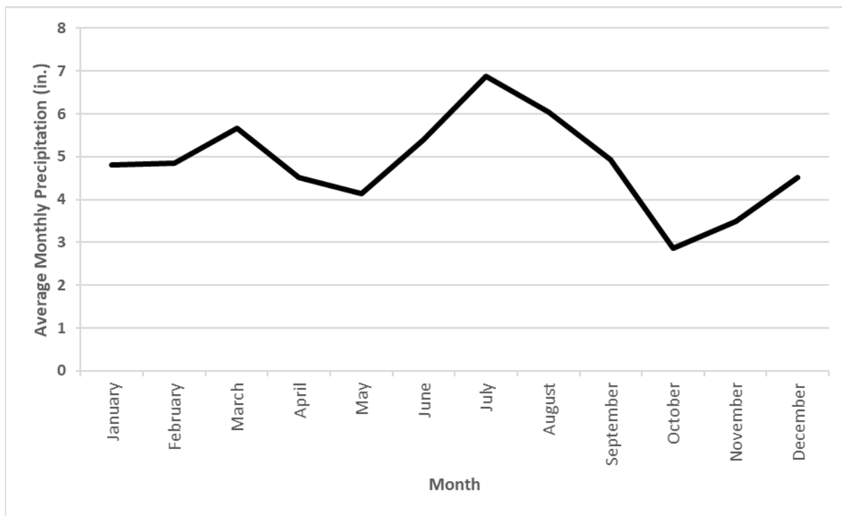
Figure 4-2. Monthly precipitation averages for NWS Station USC00081544, located in Chipley, FL.
