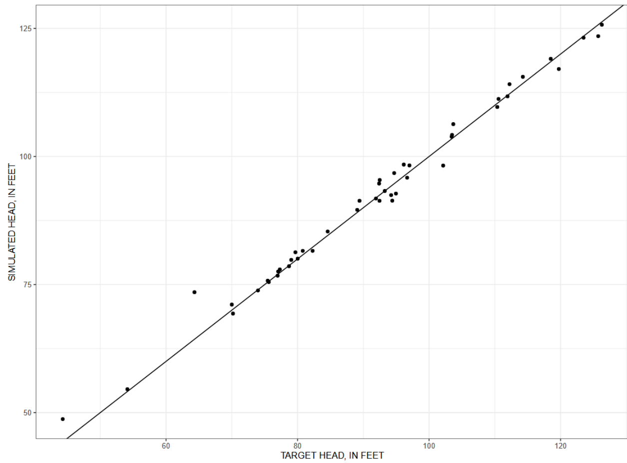
Figure 6-3. Plot of simulated versus calibration target values of groundwater levels.
