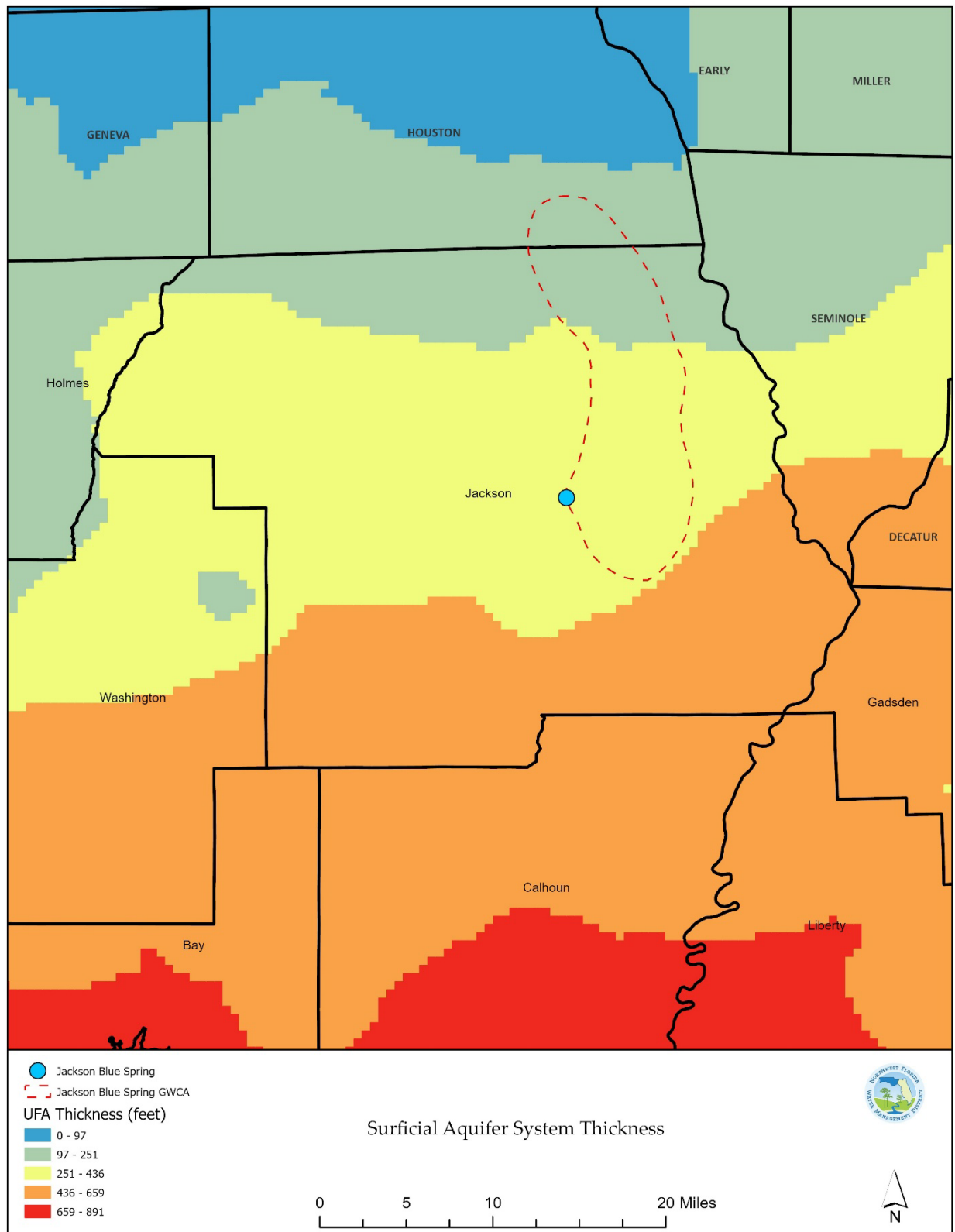
Figure 2-13. Upper Floridan aquifer thickness
