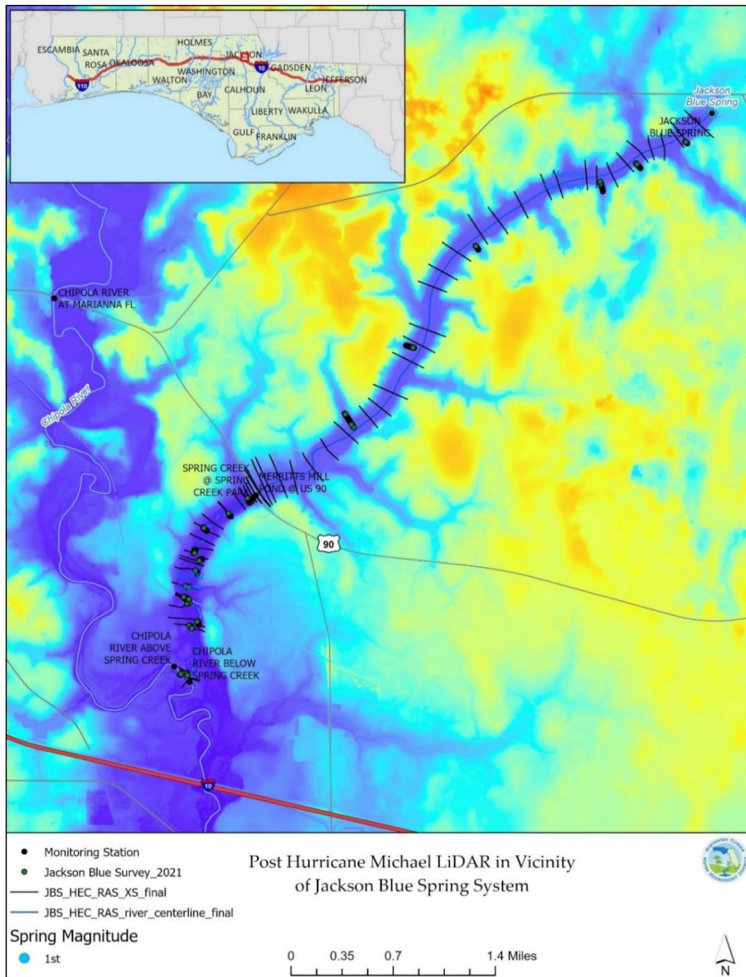
Figure 6-7. HEC-RAS model domain and Post-Hurricane Michael LiDAR-derived land surface elevations in the vicinity of Jackson Blue Spring.
