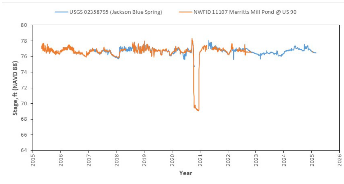
Figure 4-29. Comparison of stage at USGS 2358795 Jackson Blue Spring near Marianna with stage at NWFID 11107 Merritts Mill Pond at US 90.
