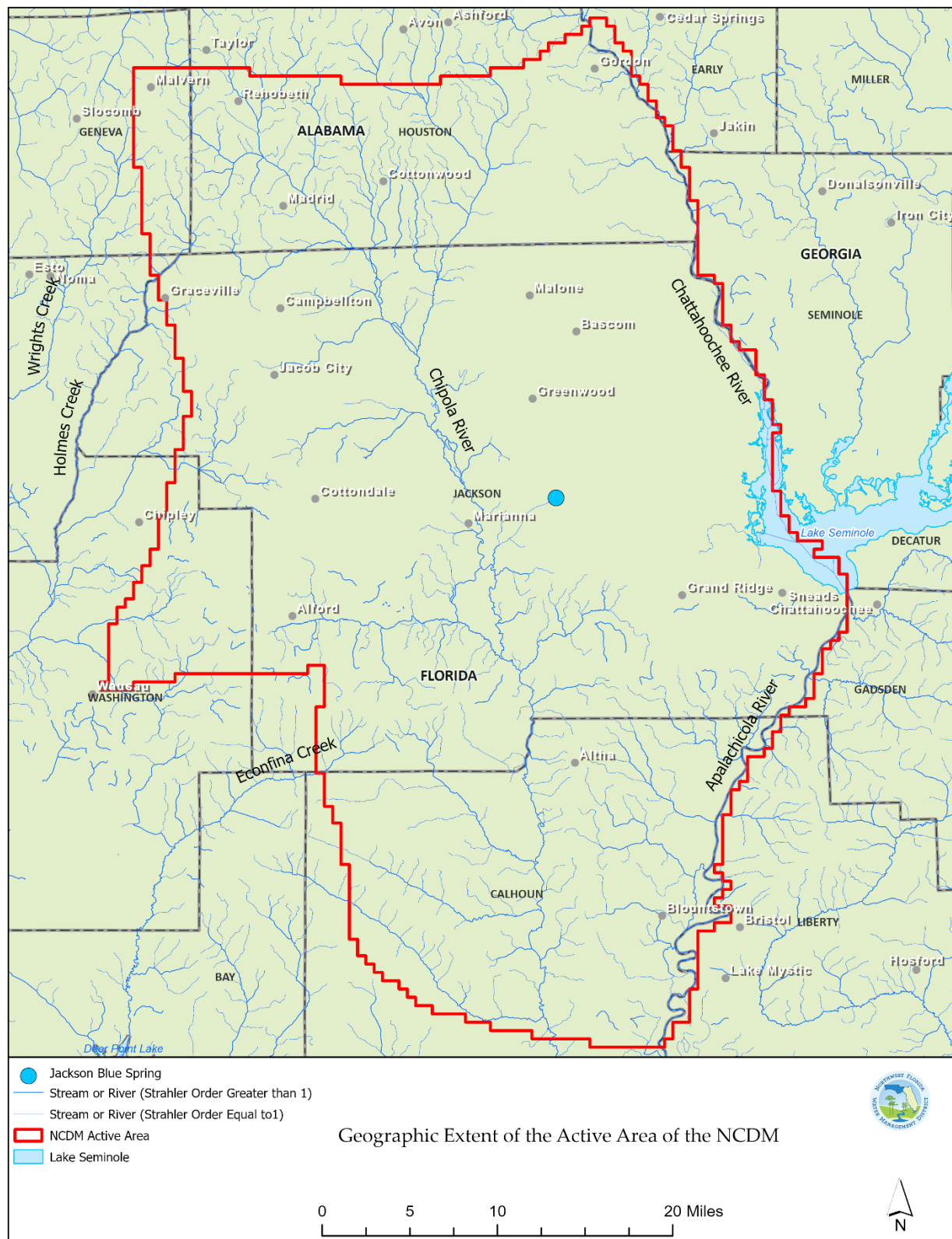
Figure 6-1. Geographic extent of the NCDM groundwater flow model.
