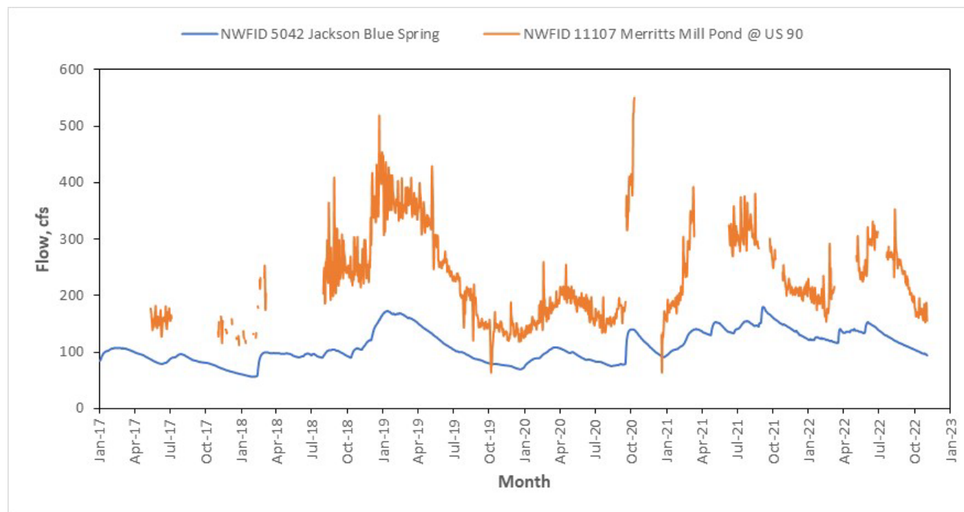
Figure 4-22. Comparison of discharge at NWFID 5042 Jackson Blue Spring with discharge at NWFID 11107 Merritts Mill Pond at US Highway 90.
