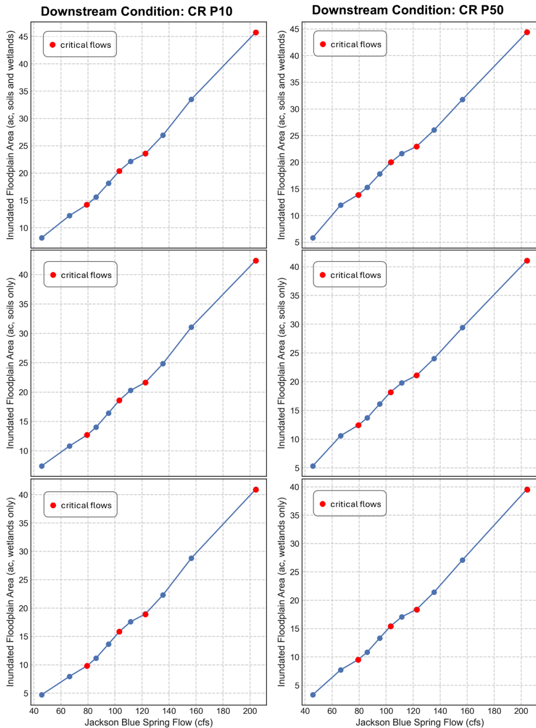
Figure 7-9. Relationships between Jackson Blue Spring flow and inundated floodplain area based on both wetlands and soils (top row), soils only (middle row), and wetlands only (bottom row) with a downstream boundary condition equal to CR P10 (left column) and CR P50 (right column).
