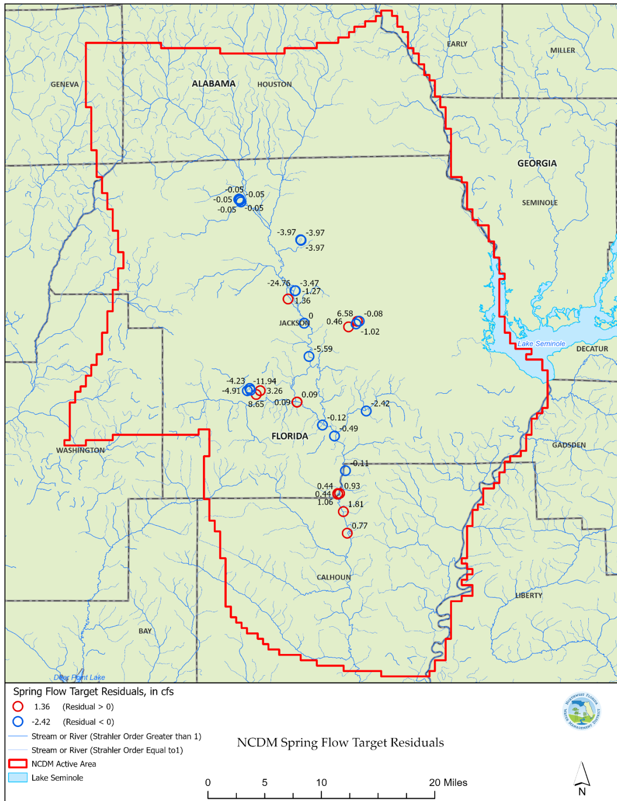
Figure 6-6. Map of differences (residuals) between simulated and calibration target values of spring flows.
