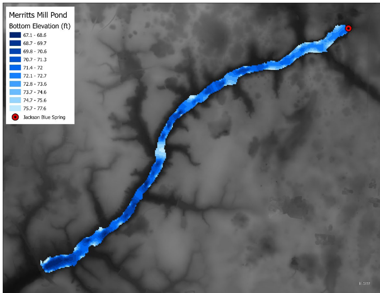
Figure 7-13. Interpolated bottom elevations within Merritts Mill Pond.
