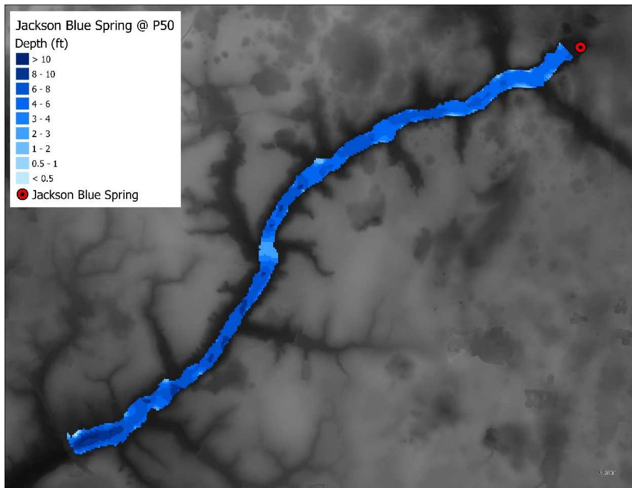
Figure 7-14. Calculated depths in Merritts Mill Pond for the P50 discharge from Jackson Blue Spring.
