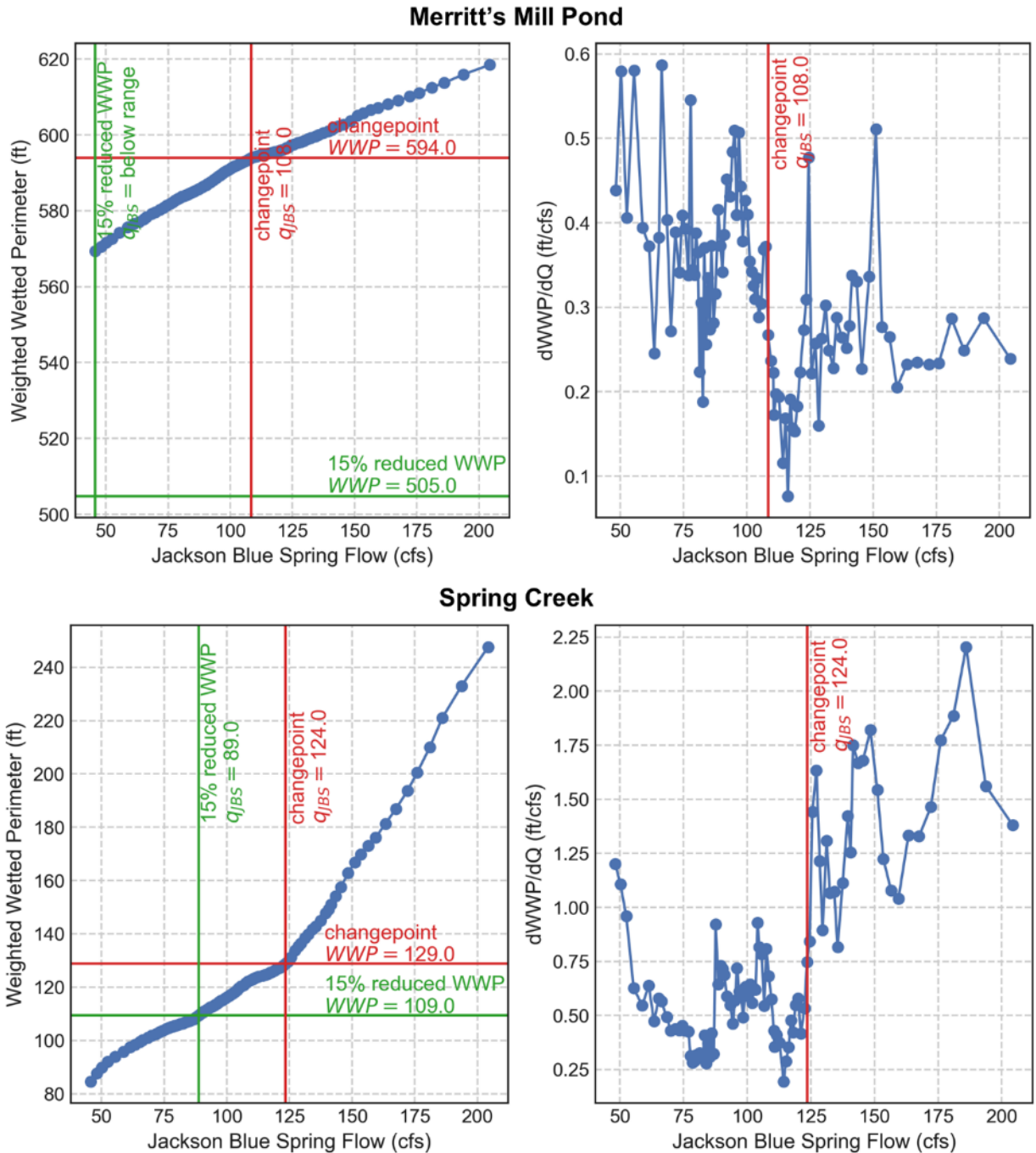
Figure 7-8. Plots showing the relationship between weighted wetted perimeter (WWP) and Jackson Blue Spring flow (left side) and the discrete first derivative of that relationship (right side) for Merritts Mill Pond (top) and Spring Creek (bottom), which were used to determine critical flows based on changepoints and flow reductions based on a 15 percent reduction in WWP.
