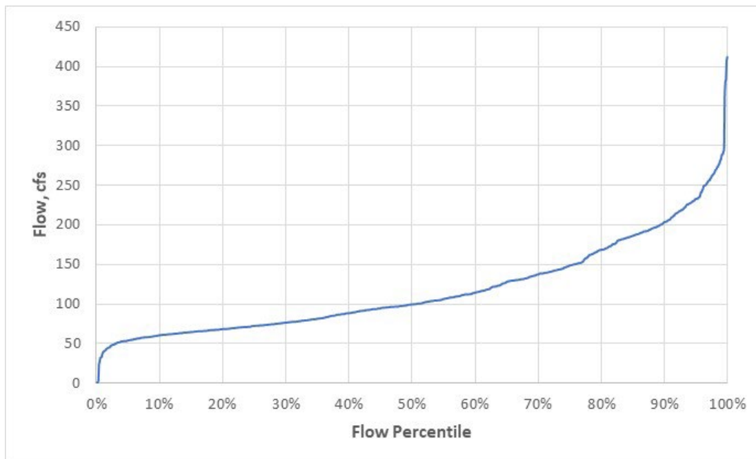
Figure 4-23. Flow duration curve of flow pickup along Merritts Mill Pond between Jackson Blue Spring and the downstream control structure at US Highway 90.
