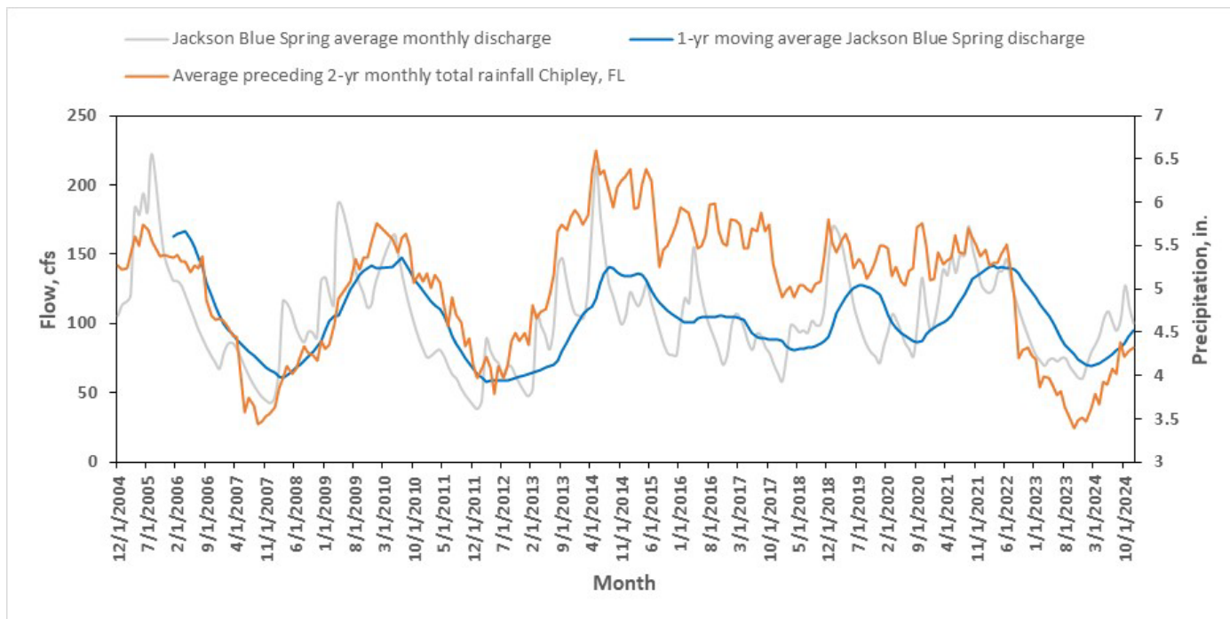
Figure 4-14. Comparison of average preceding 2-year monthly total rainfall at NWS Chipley, FL and annual average Jackson Blue Spring discharge.
