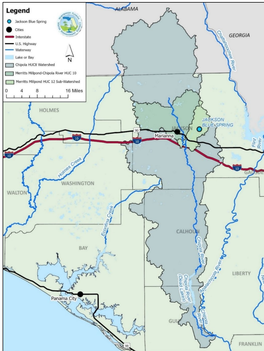
Figure 2-9. Level 8, 10, and 12 hydrologic unit code watersheds encompassing the Jackson Blue Spring study area.
