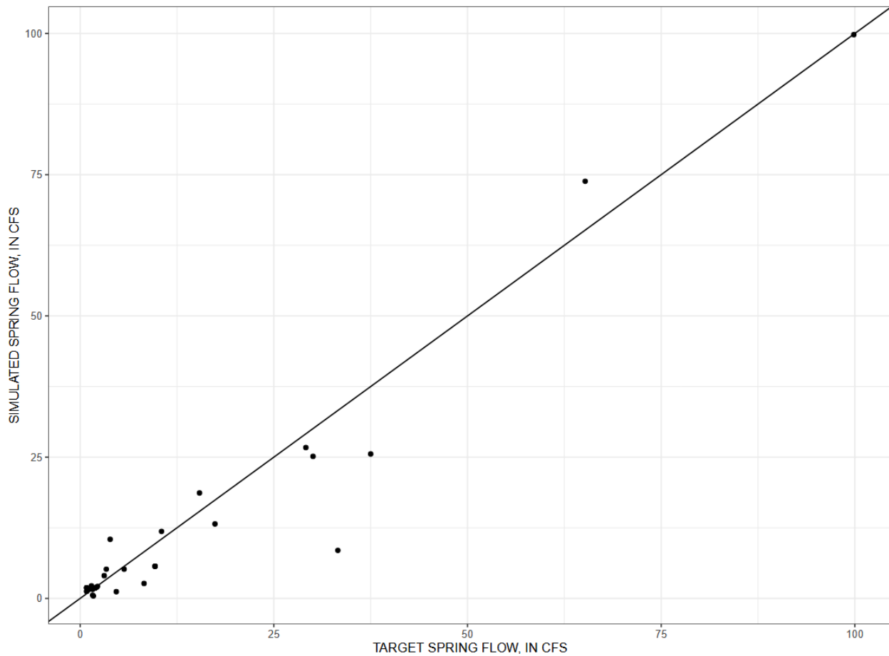
Figure 6-5. Plot of simulated versus calibration target values of spring flows.
