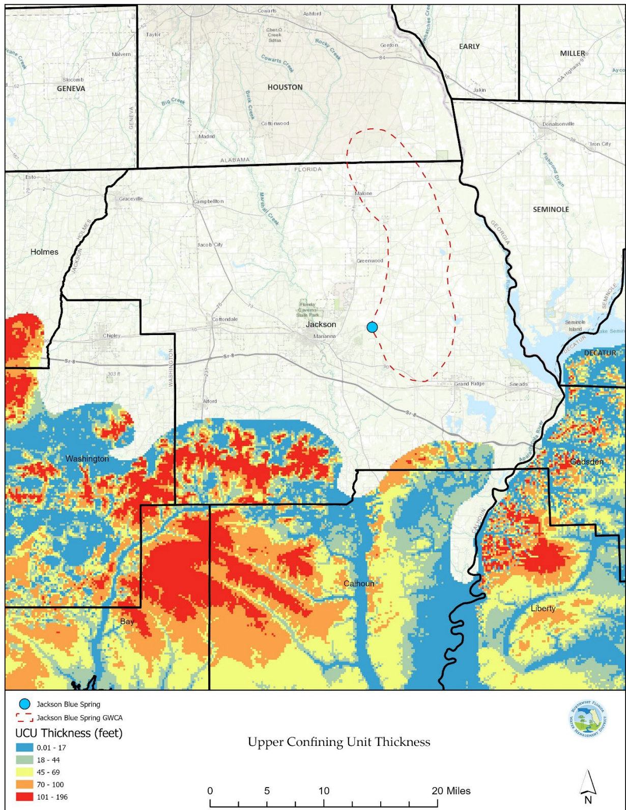
Figure 2-12. Upper confining unit thickness
