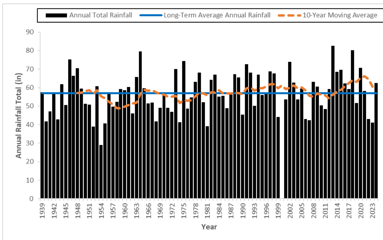
Figure 4-1. Annual precipitation totals and long-term annual average precipitation for NWS Station USC00081544, located in Chipley, FL.
