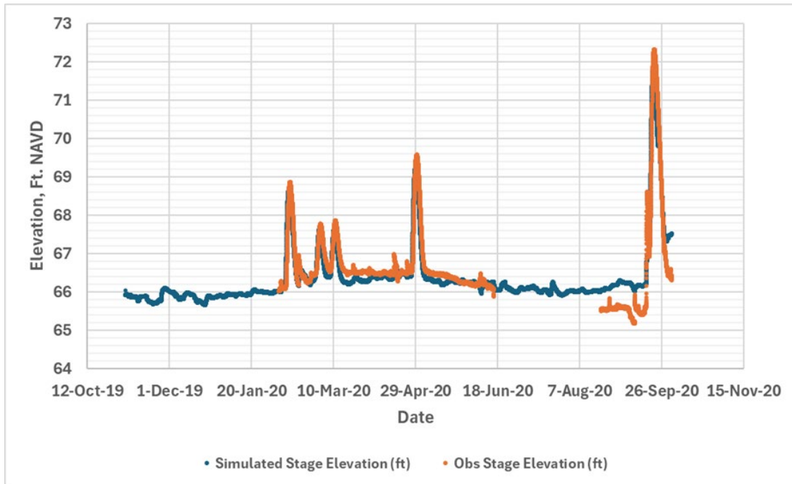
Figure 6-11. Stage time series plot for the calibration simulation, comparing observed and simulated stages at the Spring Creek @ Spring Creek Park gage.
