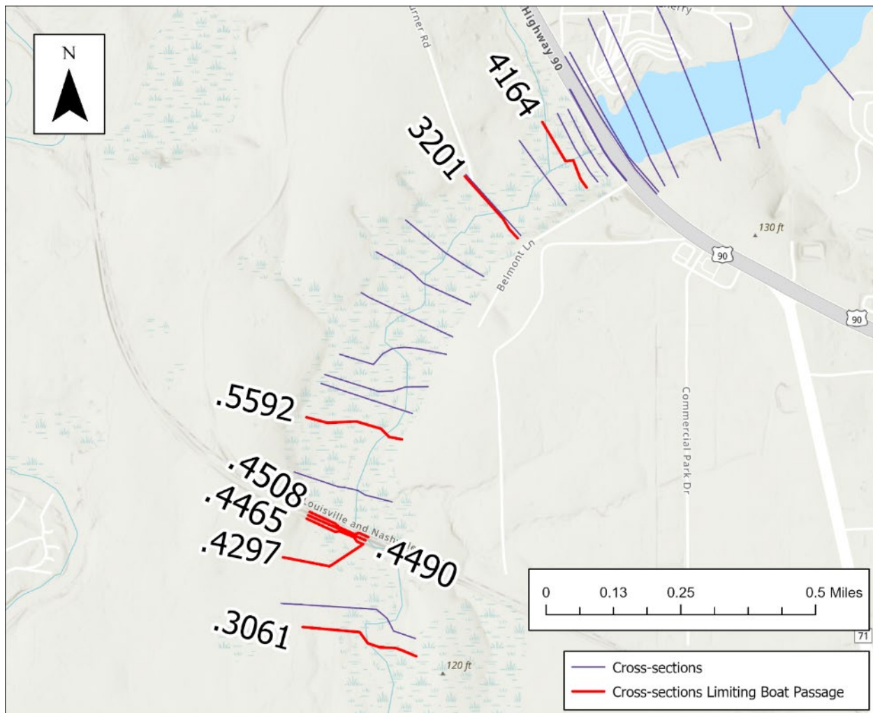
Figure 7-7. Map showing the eight cross sections with limiting critical flows for motorboat passage on Spring Creek.
