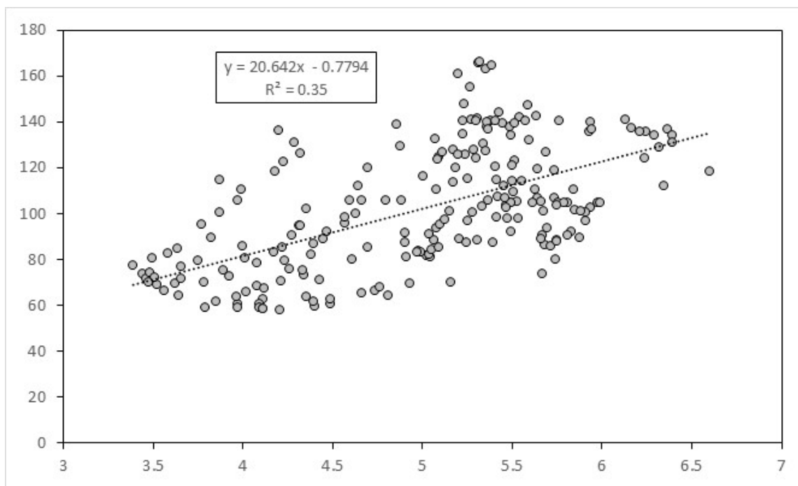
Figure 4-15. Linear regression between average preceding 2-year monthly total rainfall at NWS Chipley, FL and annual average Jackson Blue Spring discharge.
