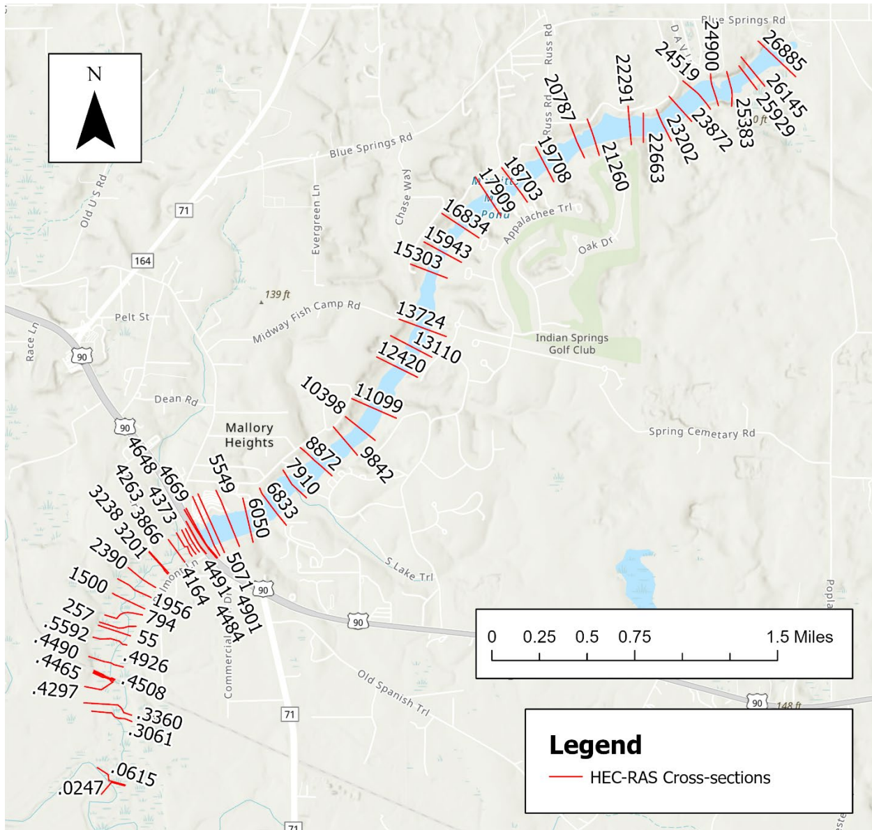
Figure 7-5. Locations of HEC-RAS cross sections labelled with identifiers used in the model.
