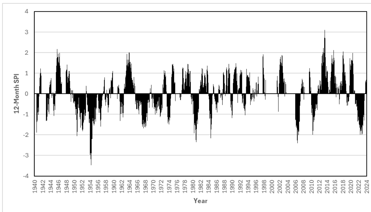
Figure 4-3. Twelve month standard precipitation index for NWS Station USC00081544, located in Chipley, FL.
