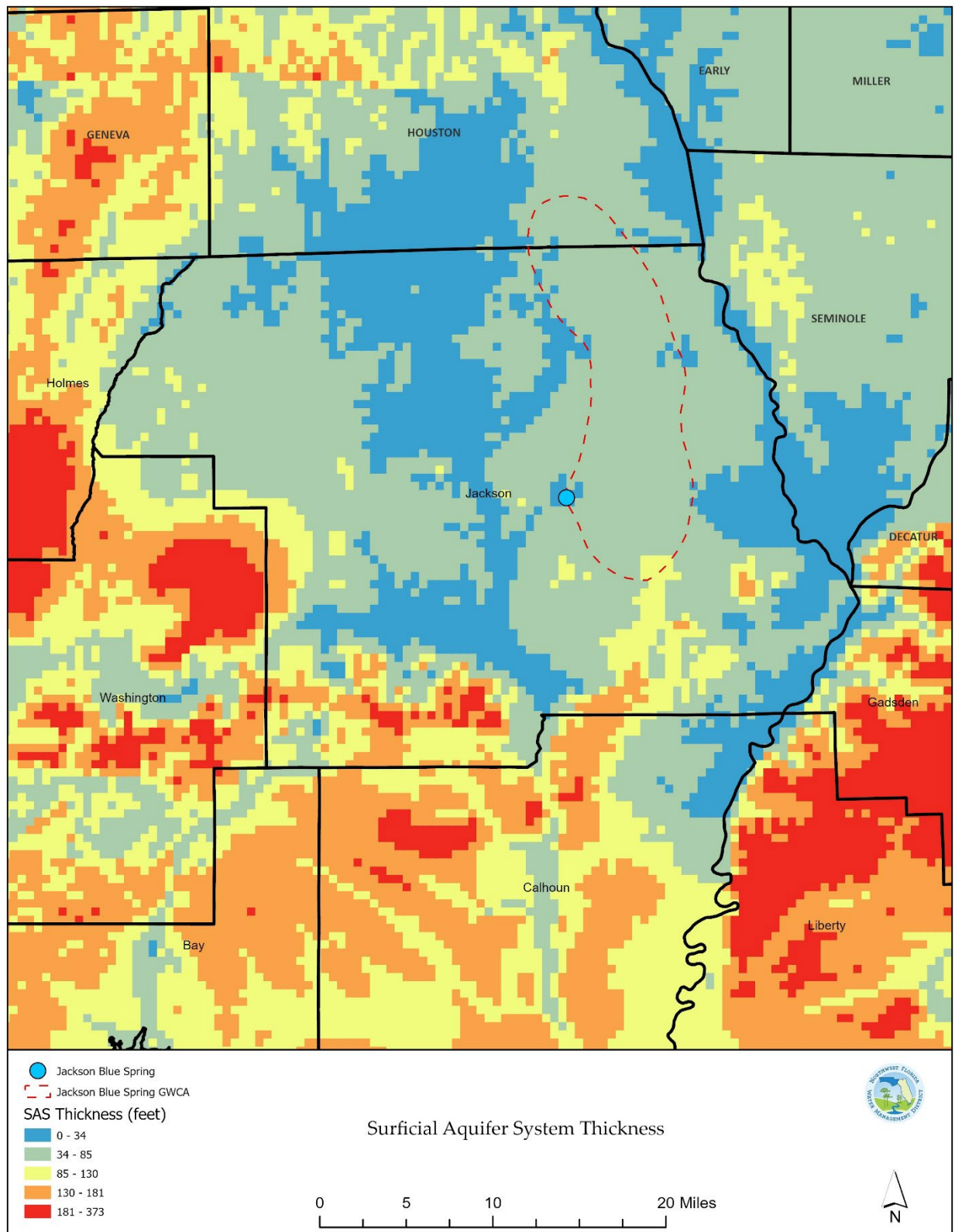
Figure 2-11. Surficial aquifer system thickness.
