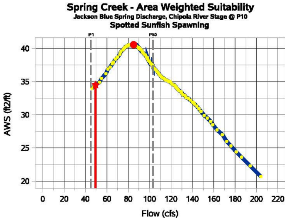
Figure 7-11. Relationship between flow and AWS for spotted sunfish spawning.
