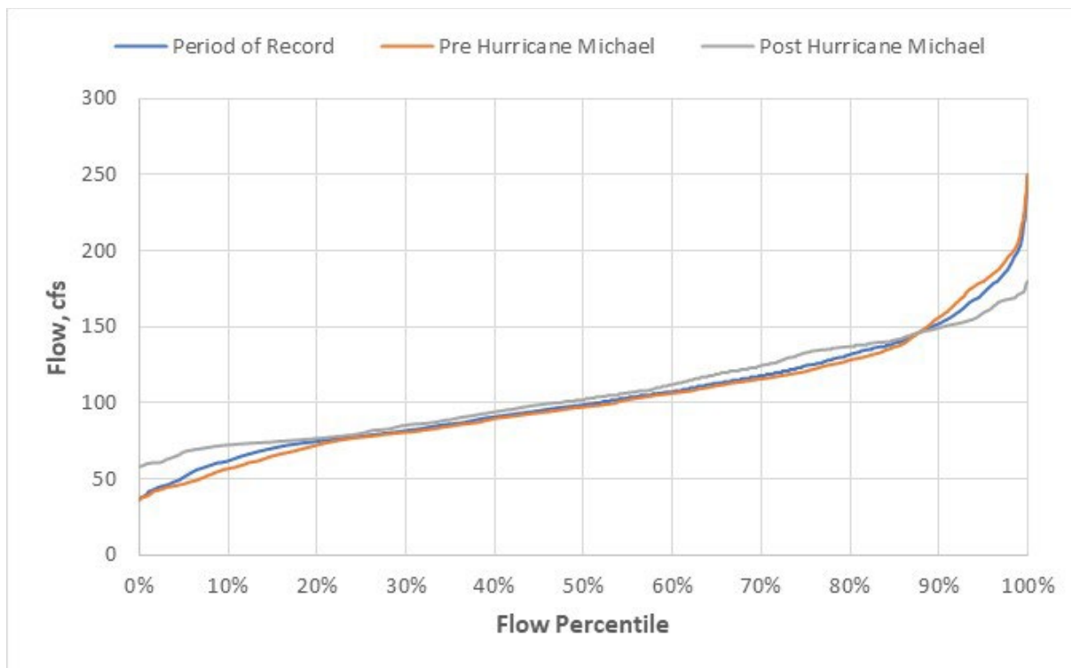
Figure 4-8. Jackson Blue Spring Discharge flow duration curves.
