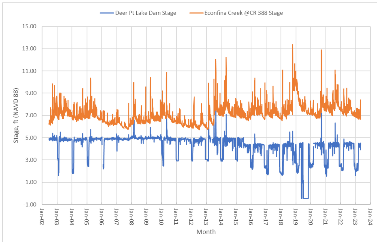
Figure 2-9. Comparison of Deer Point Lake levels with Econfina Creek Stage
