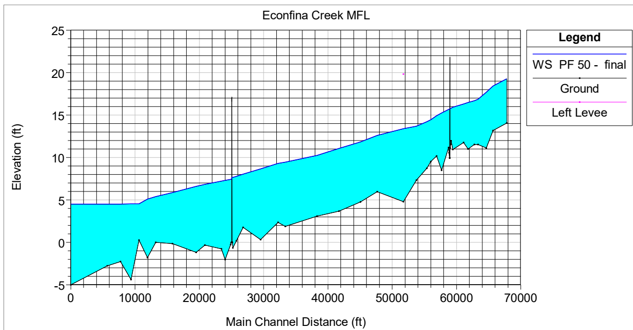
Figure 3-6. Final calibrated water surface profile
