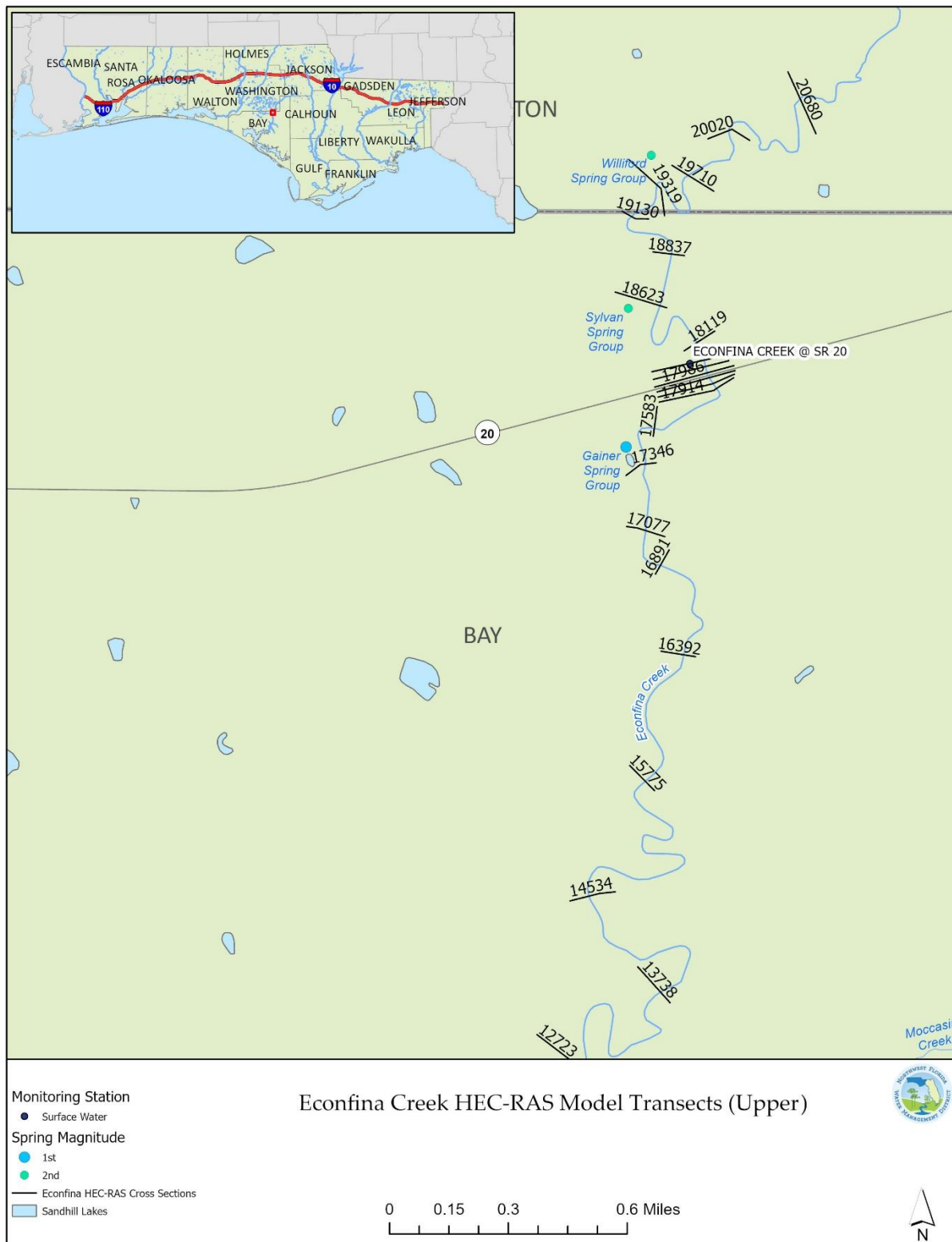
Figure 1-3b. Econfinia Creek and Springs MFL HEC-RAS Model Extent– Upper Creek
