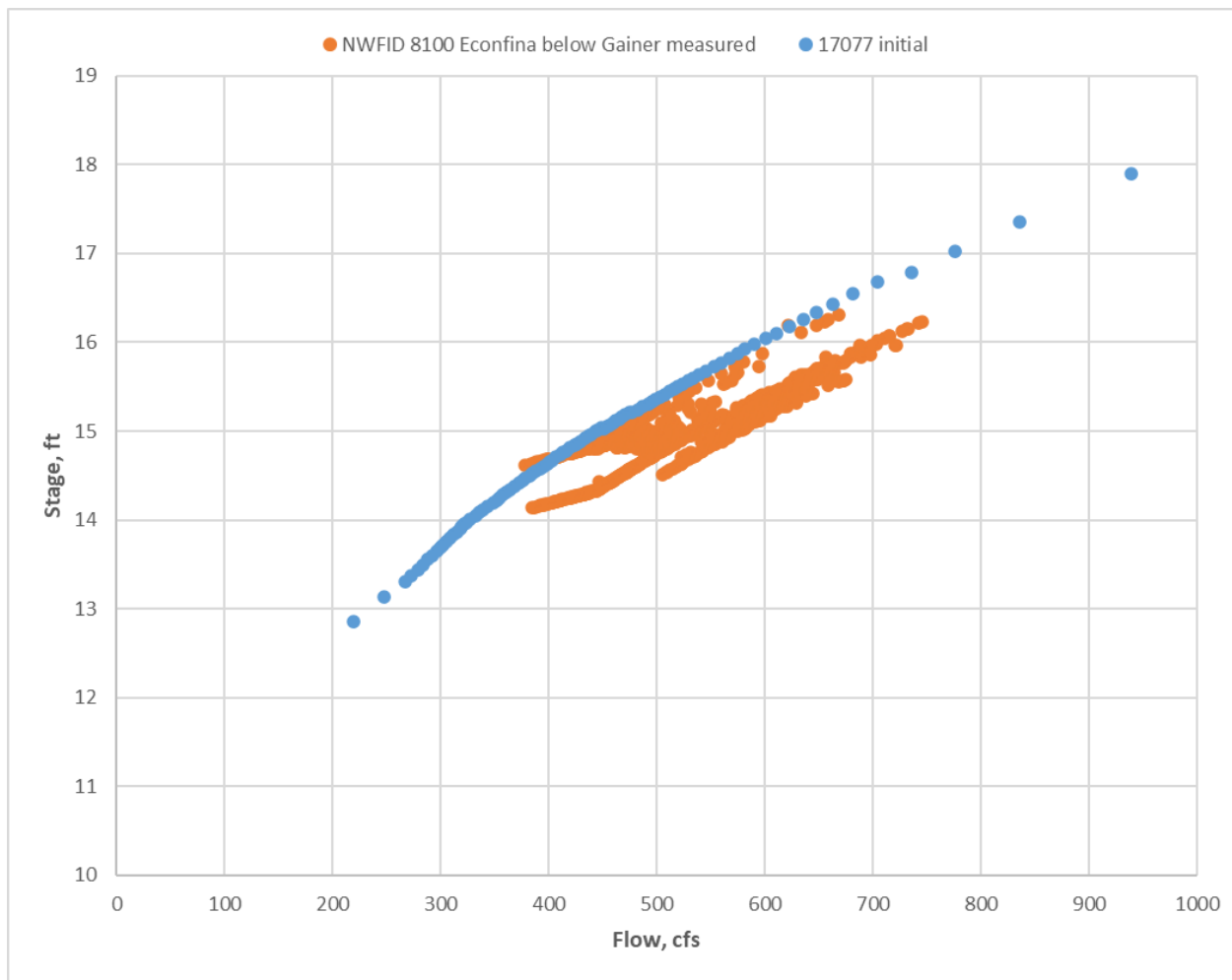
Figure 3-4. Comparison of measured stage-discharge rating at NFWMD 8100 (Econfina Creek Below Gainer Spring Group) with initial simulated stage-discharge rating at XS 17077 (nearest XS to Econfina Creek Below Gainer Spring Group)
